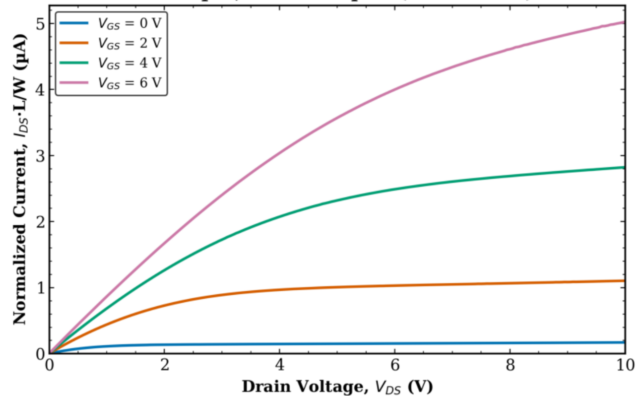
TFT1 Combined (Tr. 1 & 2) L = 8 \mu\text{m} , W = 500 \mu\text{m} (normalized)
