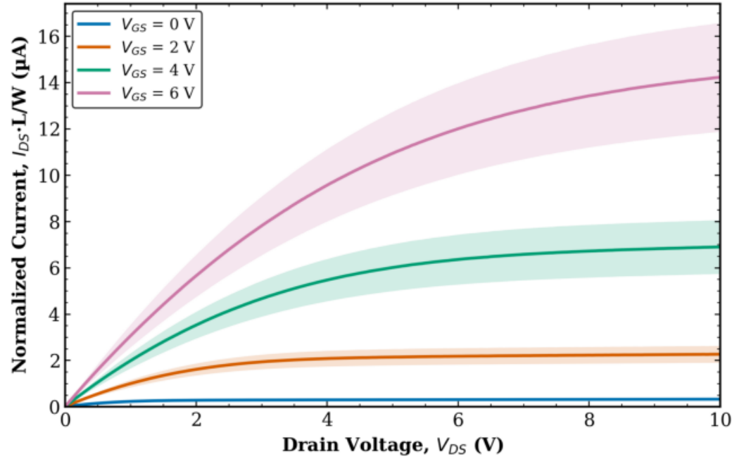
TFT1 Combined (Tr. 1 & 2) L = 20 \mu\text{m} , W = 10 \mu\text{m} (normalized)
