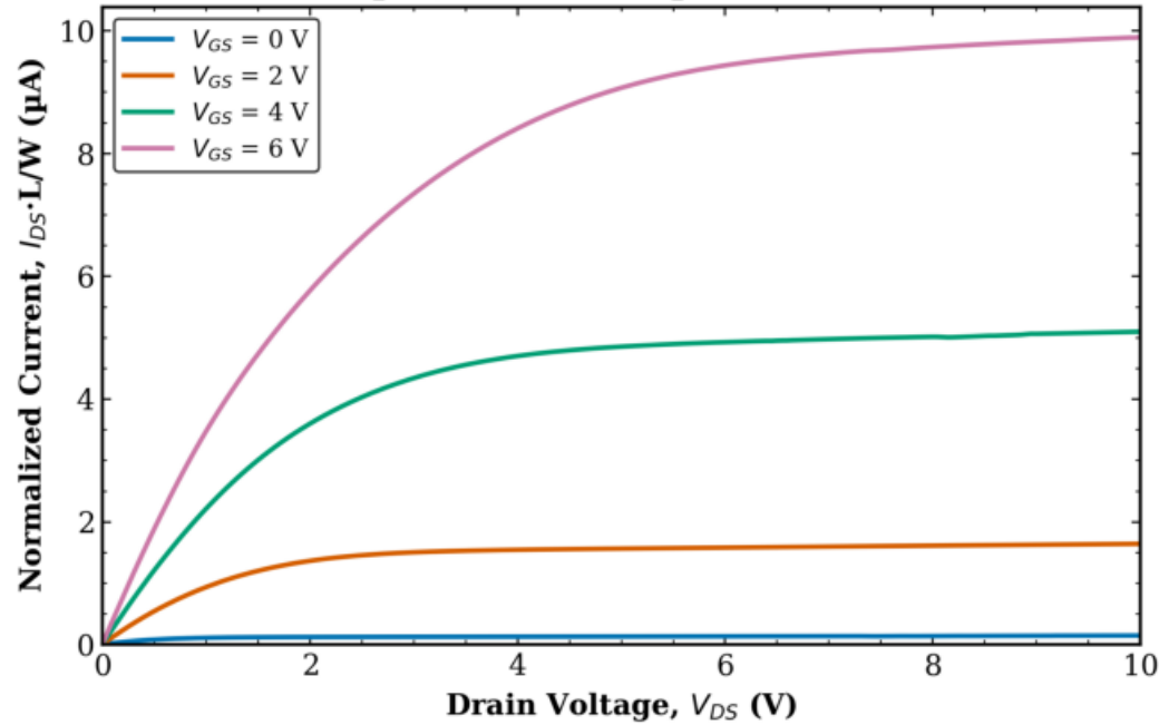
TFT1 Combined (Tr. 1 & 2) L = 20 \mu\text{m} , W = 1000 \mu\text{m} (normalized)
