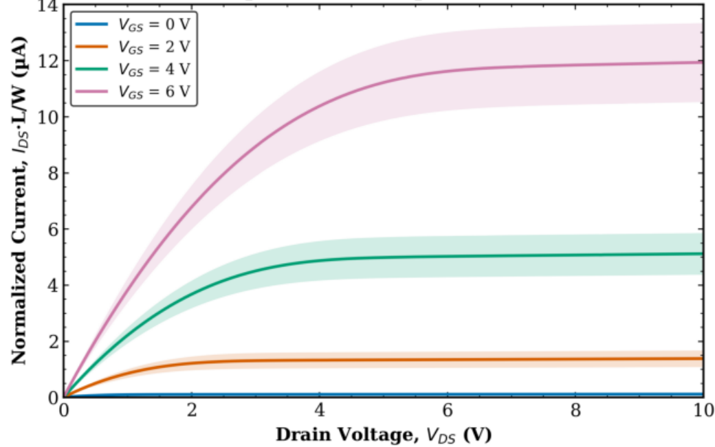
TFT1 Combined (Tr. 1 & 2) L = 160 \mu\text{m} , W = 100 \mu\text{m} (normalized)
