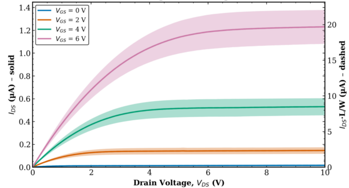
TFT1 Combined (Tr. 1 & 2) L = 160 \mu\text{m} , W = 10 \mu\text{m}
