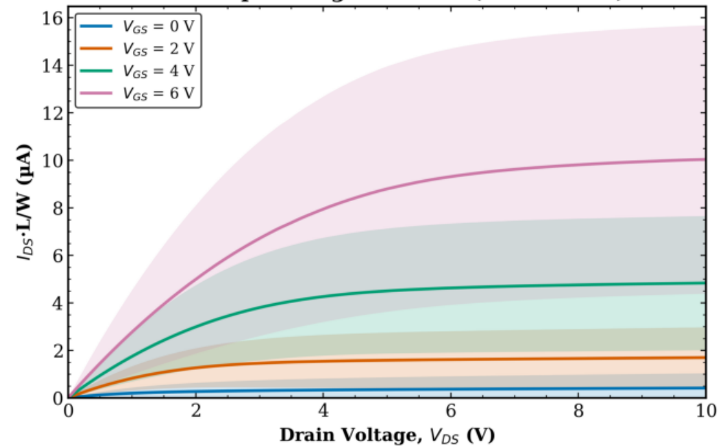
TFT1 Combined (Tr. 1 & 2) W = 50 \mu\text{m} - avg over all L (mean \pm std)
