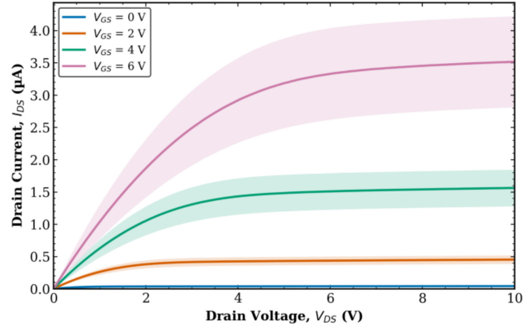
TFT1 Combined (Tr. 1 & 2) L = 40 \mu\text{m} , W = 10 \mu\text{m}
