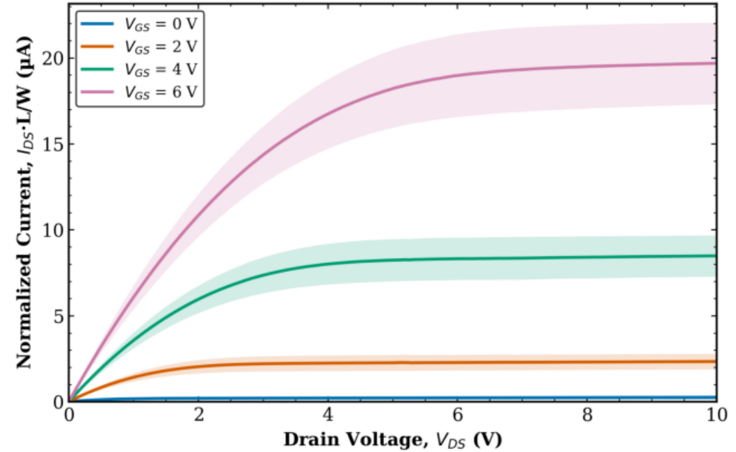
TFT1 Combined (Tr. 1 & 2) L = 160 \mu\text{m} , W = 10 \mu\text{m} (normalized)
