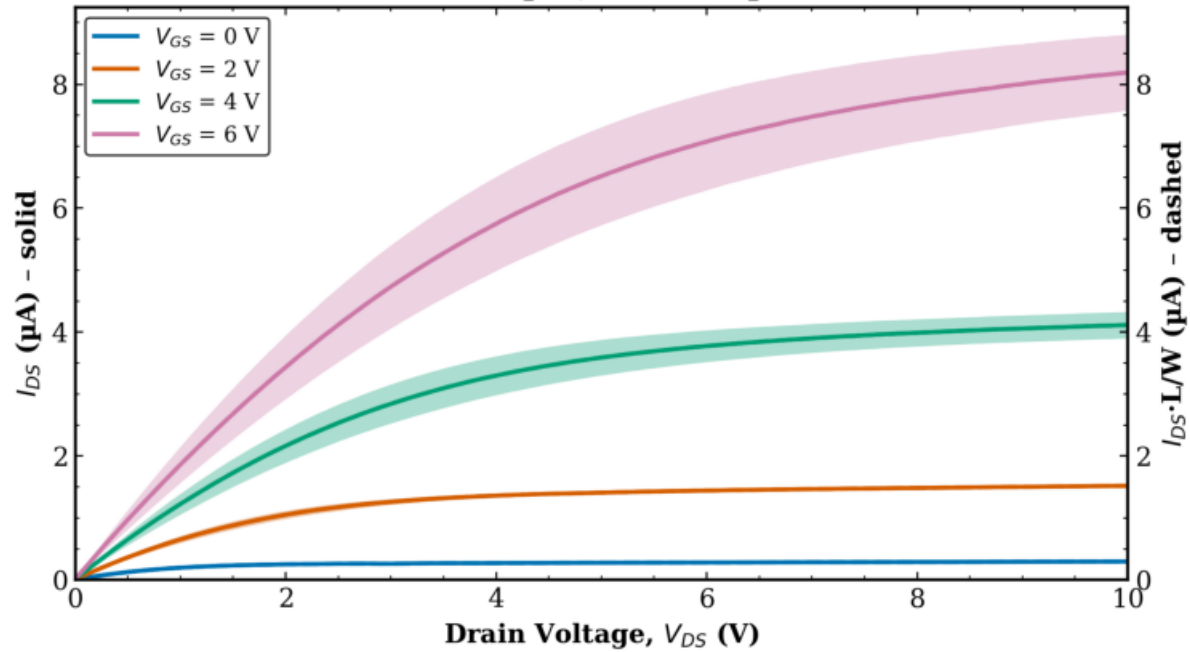
TFT1 Combined (Tr. 1 & 2) L = 10 \mu\text{m} , W = 10 \mu\text{m}
