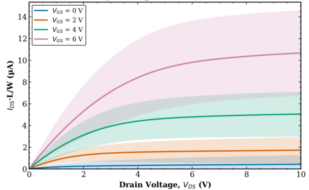
TFT1 Combined (Tr. 1 & 2) W = 100 \mu\text{m} - avg over all L (mean \pm std)
