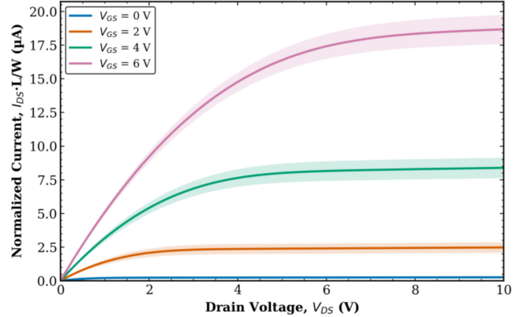
TFT1 Combined (Tr. 1 & 2) L = 80 \mu\text{m} , W = 10 \mu\text{m} (normalized)
