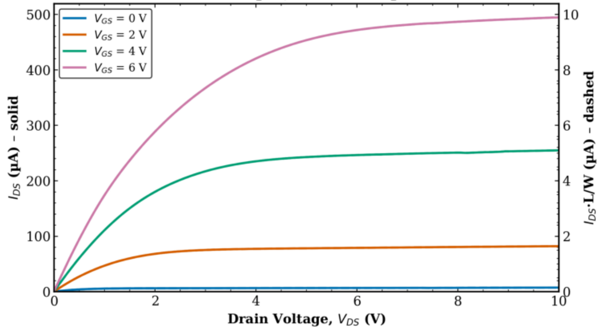
TFT1 Combined (Tr. 1 & 2) L = 20 \mu\text{m} , W = 1000 \mu\text{m}
