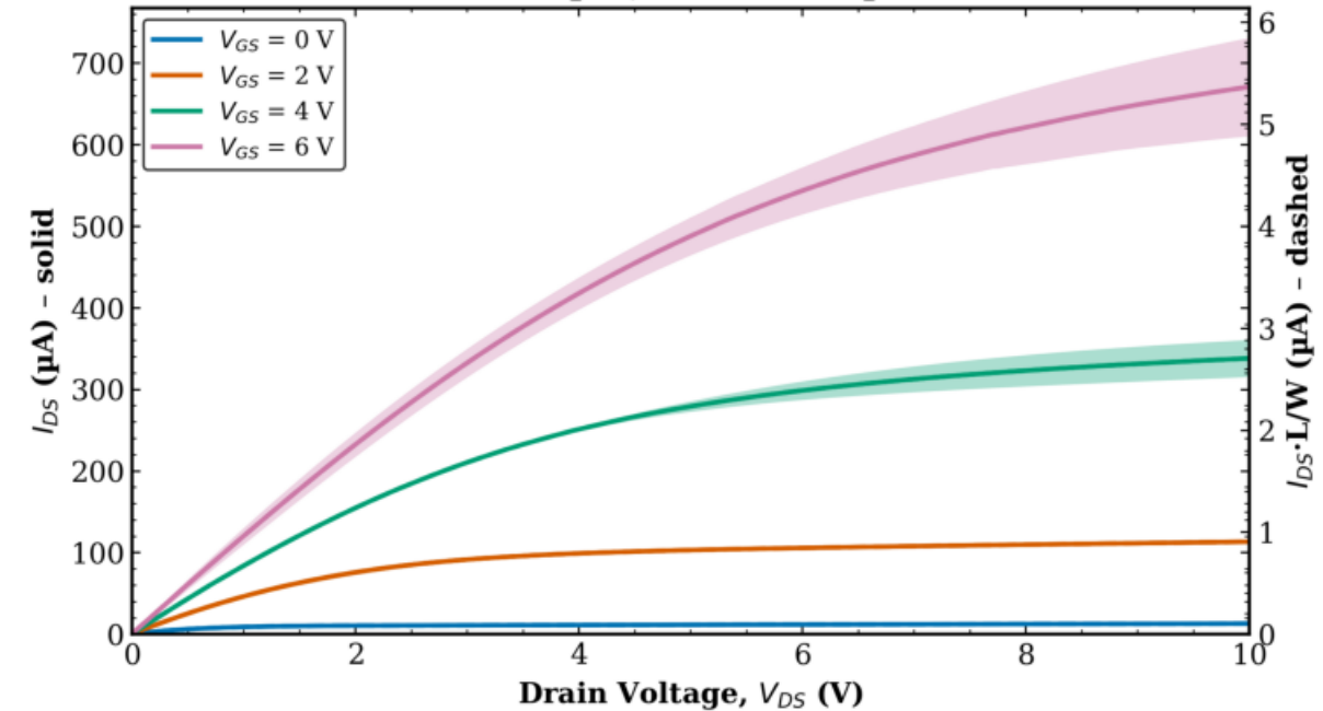
TFT1 Combined (Tr. 1 & 2) L = 8 \mu\text{m} , W = 1000 \mu\text{m}
