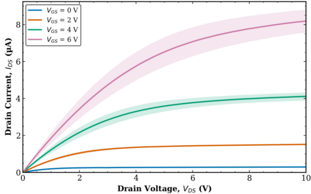
TFT1 Combined (Tr. 1 & 2) L = 10 \mu\text{m} , W = 10 \mu\text{m}
