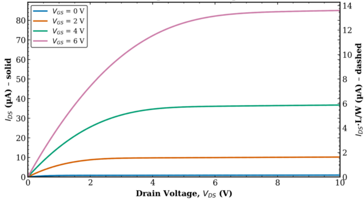
TFT1 Combined (Tr. 1 & 2) L = 80 \mu\text{m} , W = 500 \mu\text{m}
