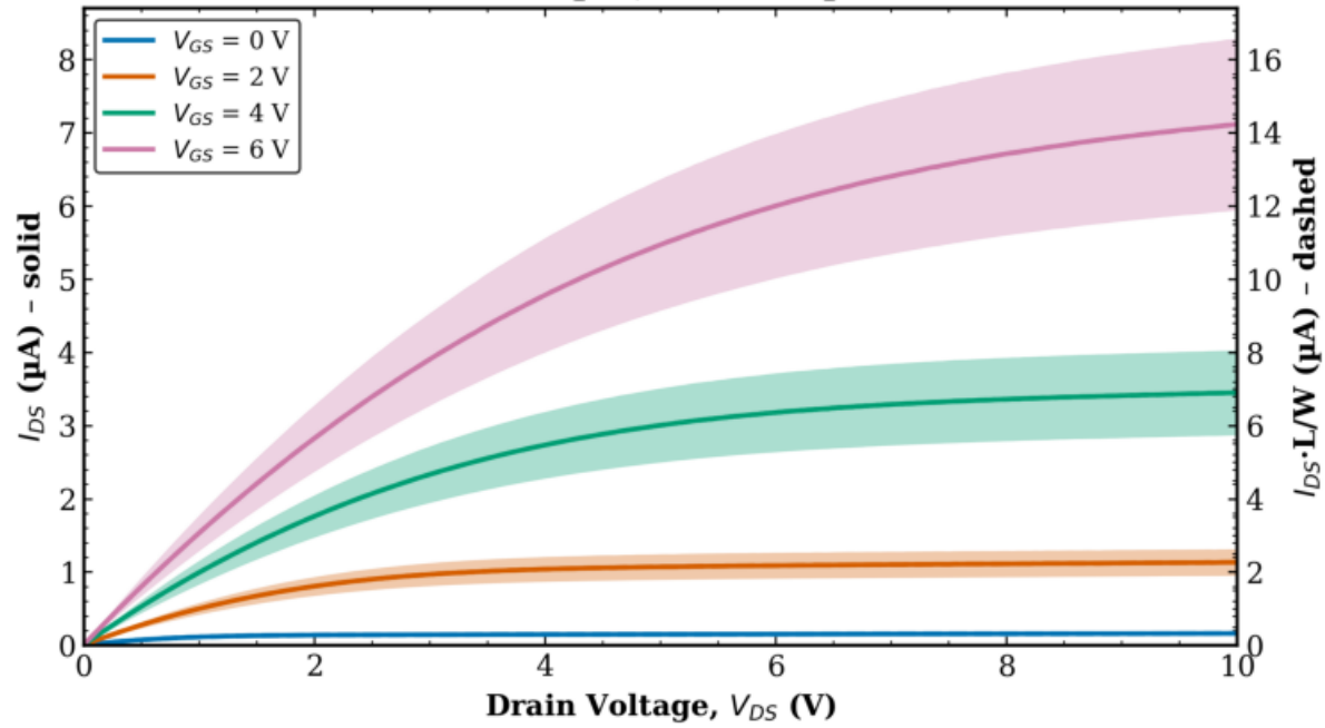
TFT1 Combined (Tr. 1 & 2) L = 20 \mu\text{m} , W = 10 \mu\text{m}
