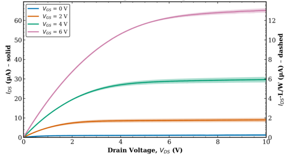
TFT1 Combined (Tr. 1 & 2) L = 20 \mu\text{m} , W = 100 \mu\text{m}
