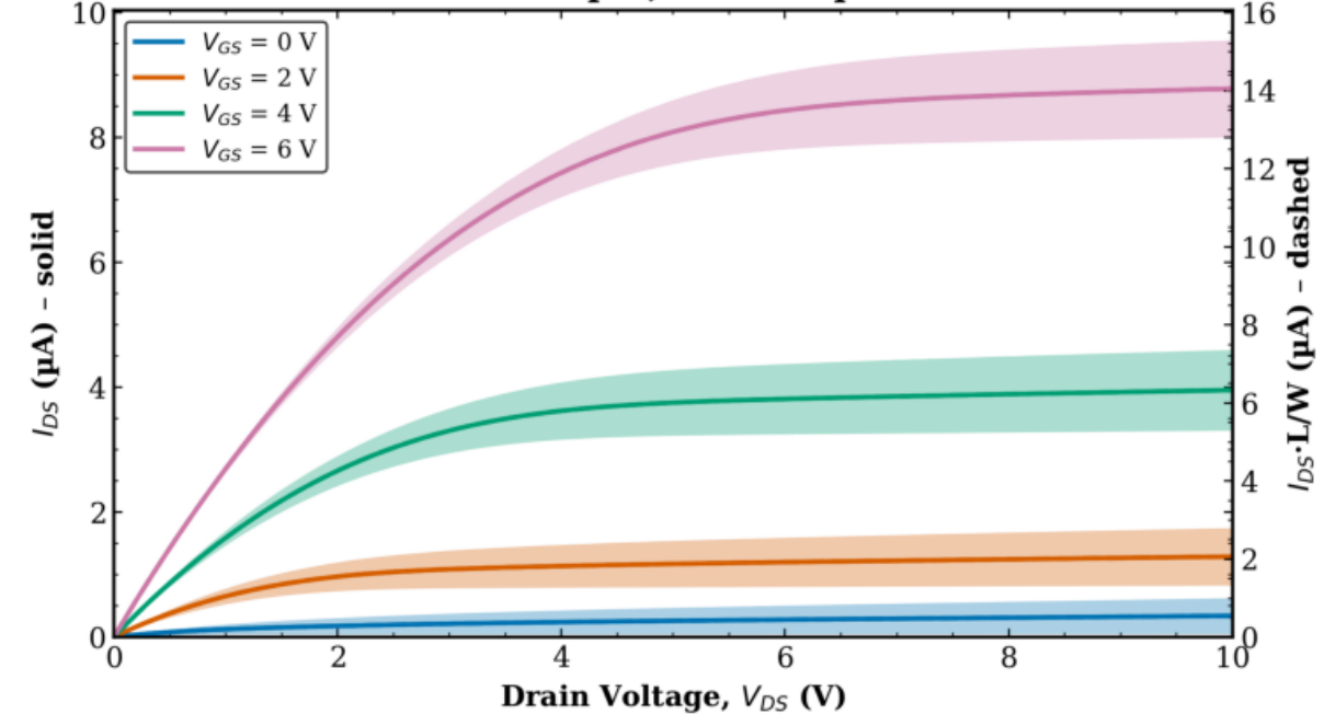
TFT1 Combined (Tr. 1 & 2) L = 80 \mu\text{m} , W = 50 \mu\text{m}
