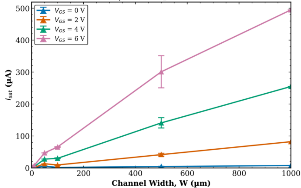
TFT1 Combined (Tr. 1 & 2) I_{sat} vs W | L = 20 \mu\text{m} (mean \pm std)
