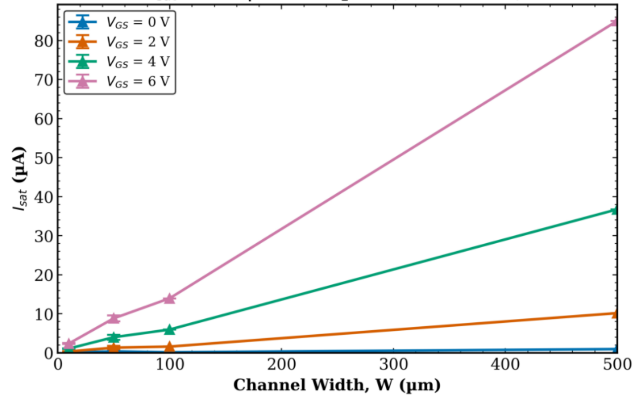
TFT1 Combined (Tr. 1 & 2) I_{sat} vs W | L = 80 \mu\text{m} (mean \pm std)
