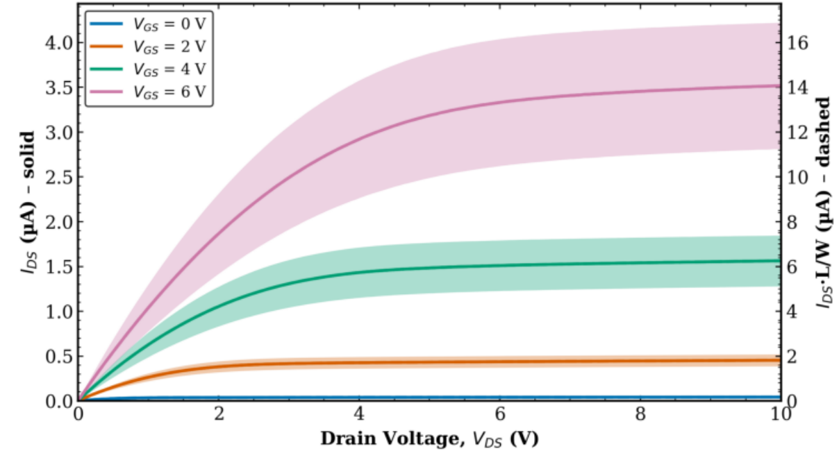
TFT1 Combined (Tr. 1 & 2) L = 40 \mu\text{m} , W = 10 \mu\text{m}
