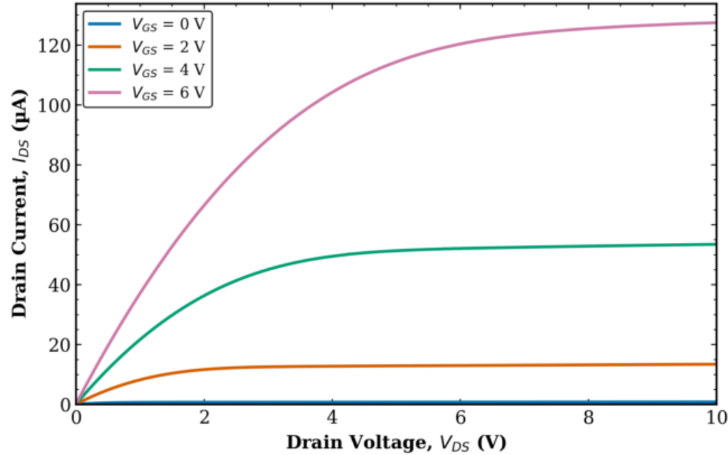
TFT1 Combined (Tr. 1 & 2) L = 40 \mu\text{m} , W = 500 \mu\text{m}
