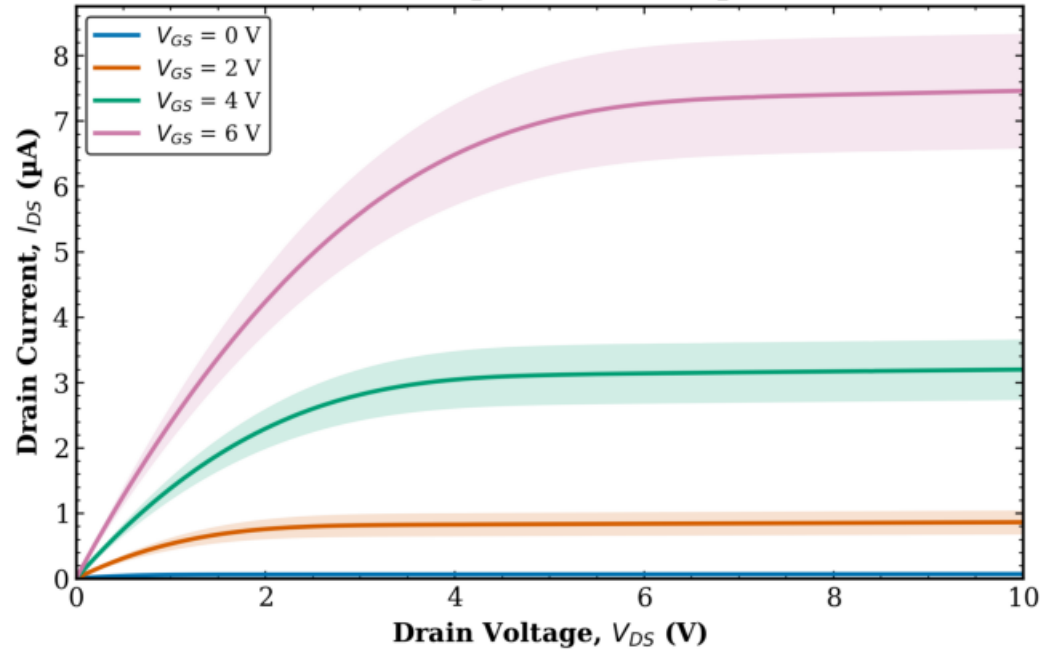
TFT1 Combined (Tr. 1 & 2) L = 160 \mu\text{m} , W = 100 \mu\text{m}
