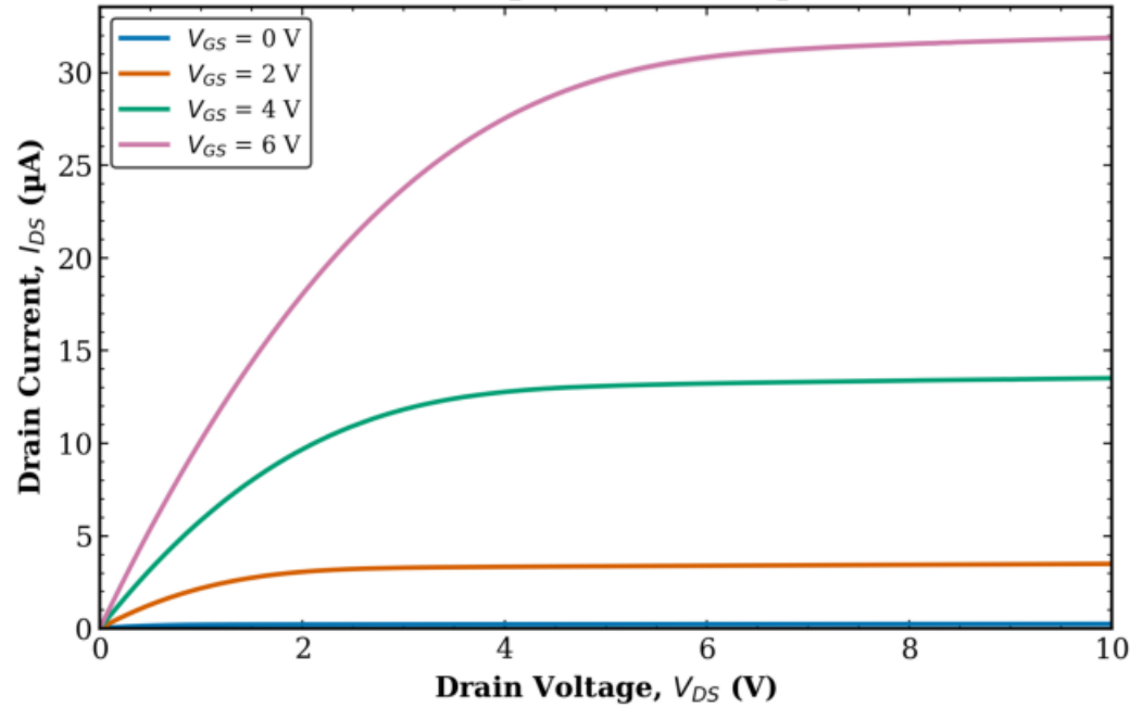
TFT1 Combined (Tr. 1 & 2) L = 40 \mu\text{m} , W = 100 \mu\text{m}
