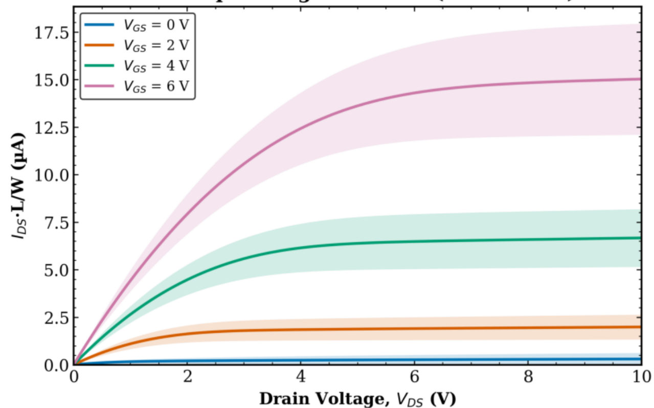
TFT1 Combined (Tr. 1 & 2) L = 80 \mu\text{m} - avg over all W (mean \pm std)
