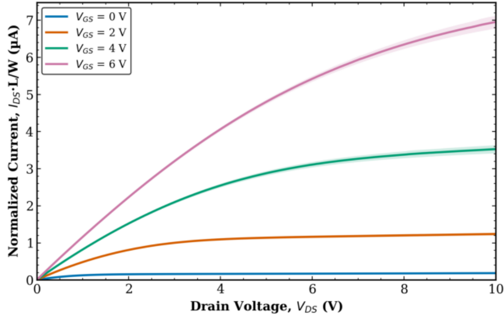
TFT1 Combined (Tr. 1 & 2) L = 10 \mu\text{m} , W = 500 \mu\text{m} (normalized)
