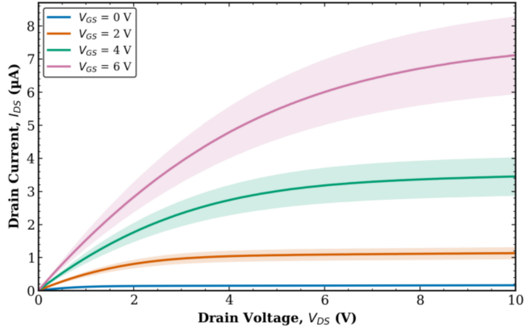
TFT1 Combined (Tr. 1 & 2) L = 20 \mu\text{m} , W = 10 \mu\text{m}
