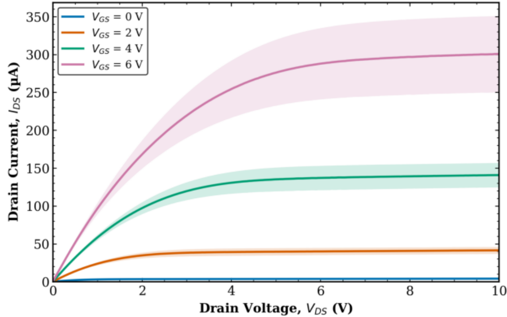
TFT1 Combined (Tr. 1 & 2) L = 20 \mu\text{m} , W = 500 \mu\text{m}
