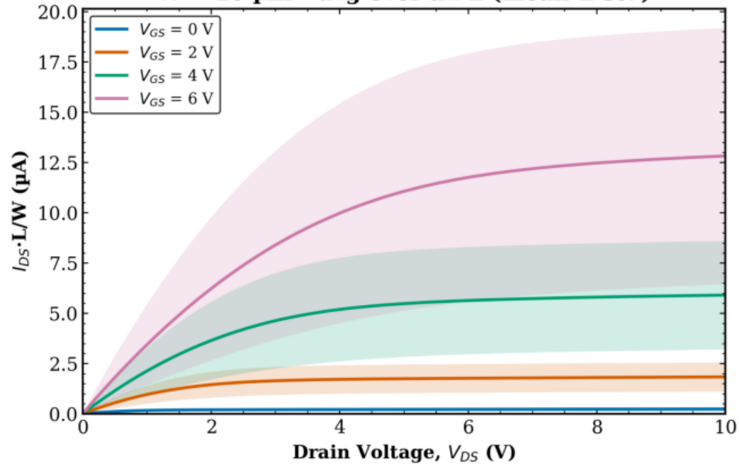
TFT1 Combined (Tr. 1 & 2) W = 10 \mu\text{m} - avg over all L (mean \pm std)
