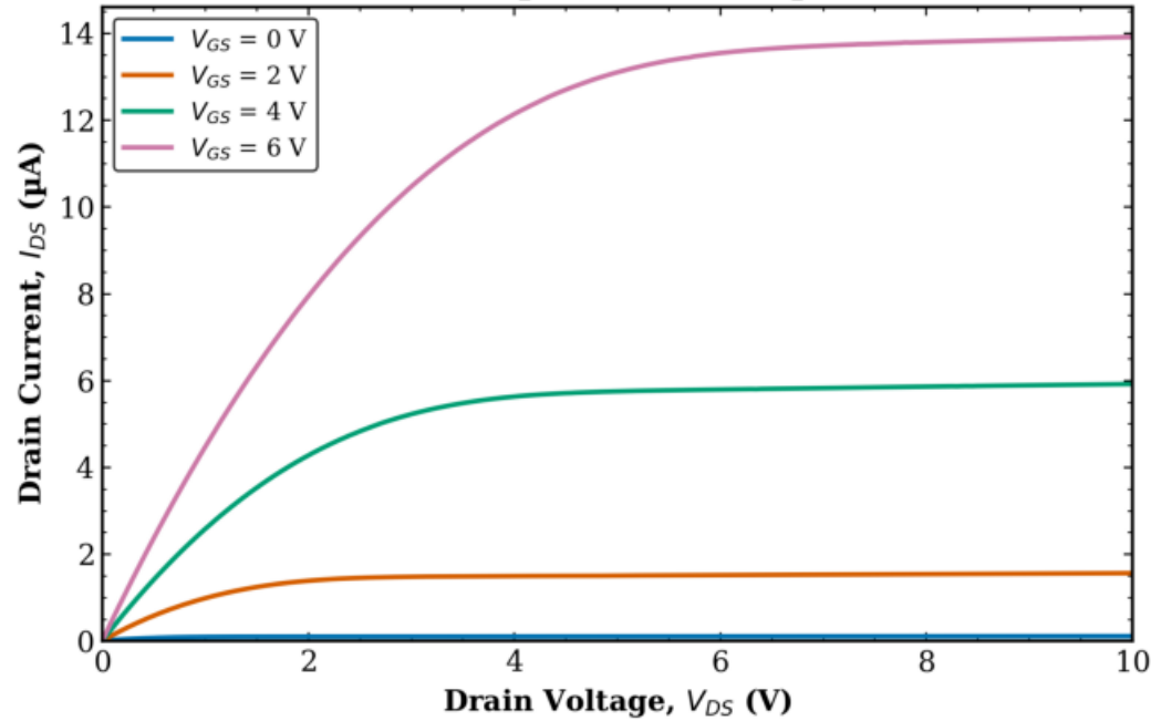
TFT1 Combined (Tr. 1 & 2) L = 80 \mu\text{m} , W = 100 \mu\text{m}
