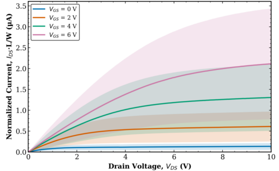
TFT1 Combined (Tr. 1 & 2) L = 8 \mu\text{m} , W = 10 \mu\text{m} (normalized)
