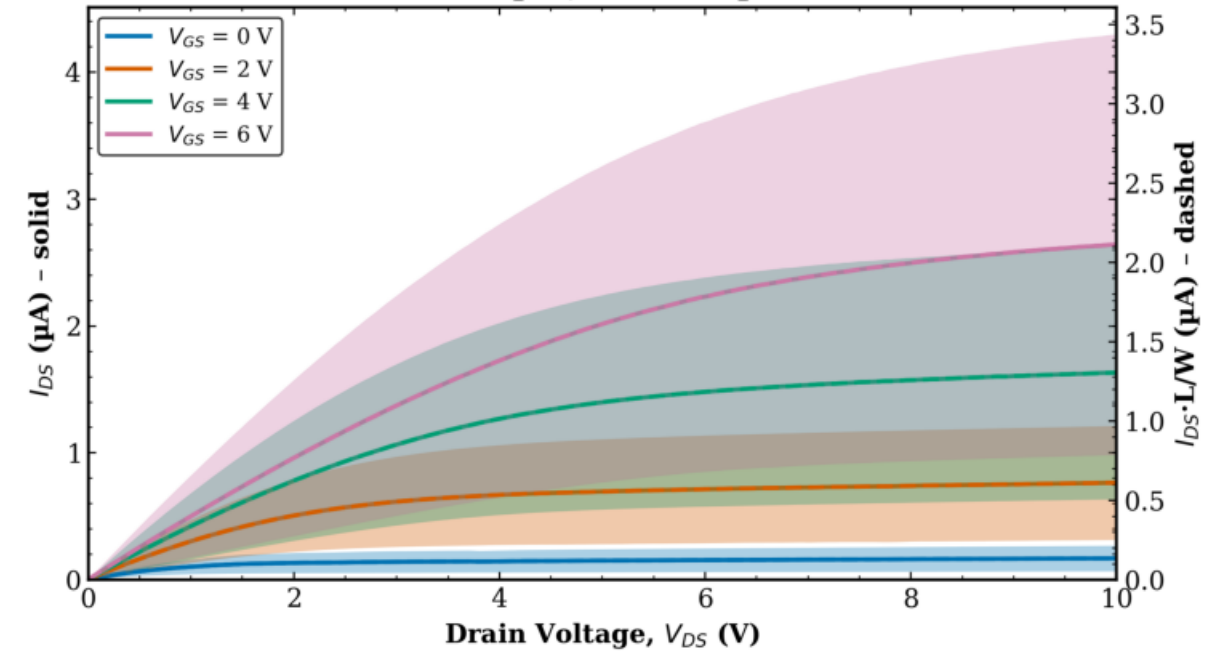
TFT1 Combined (Tr. 1 & 2) L = 8 \mu\text{m} , W = 10 \mu\text{m}
