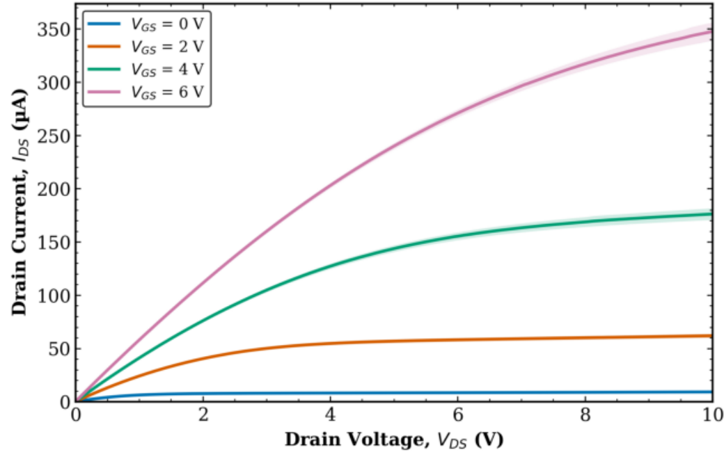
TFT1 Combined (Tr. 1 & 2) L = 10 \mu\text{m} , W = 500 \mu\text{m}
