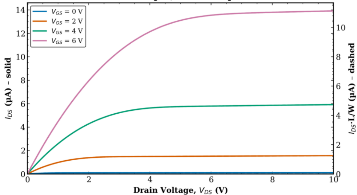
TFT1 Combined (Tr. 1 & 2) L = 80 \mu\text{m} , W = 100 \mu\text{m}
