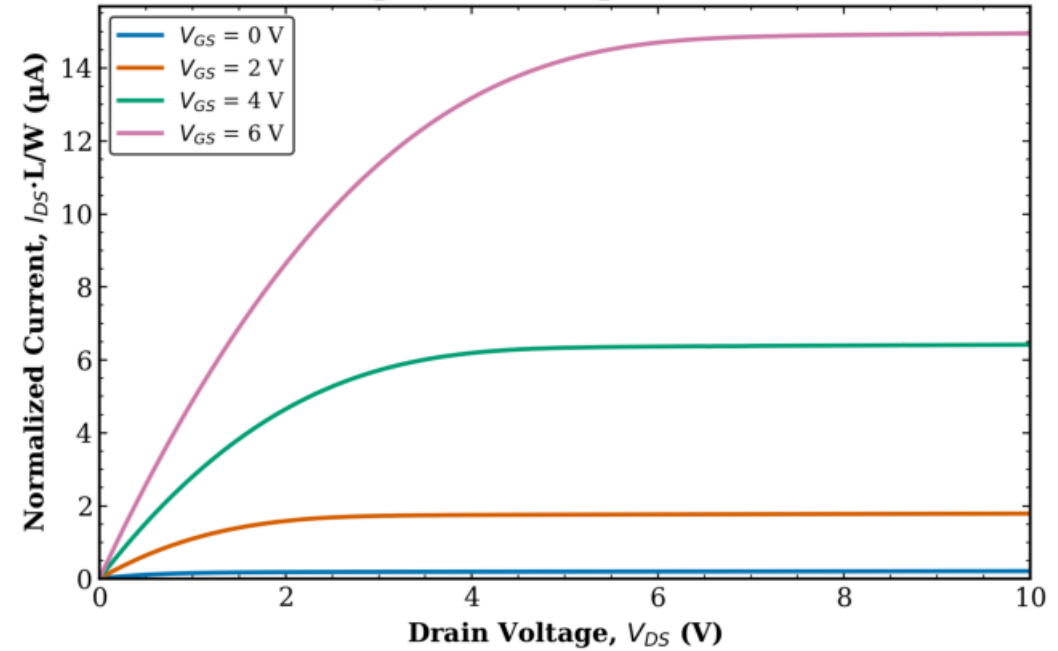
TFT1 Combined (Tr. 1 & 2) L = 160 \mu\text{m} , W = 50 \mu\text{m} (normalized)
