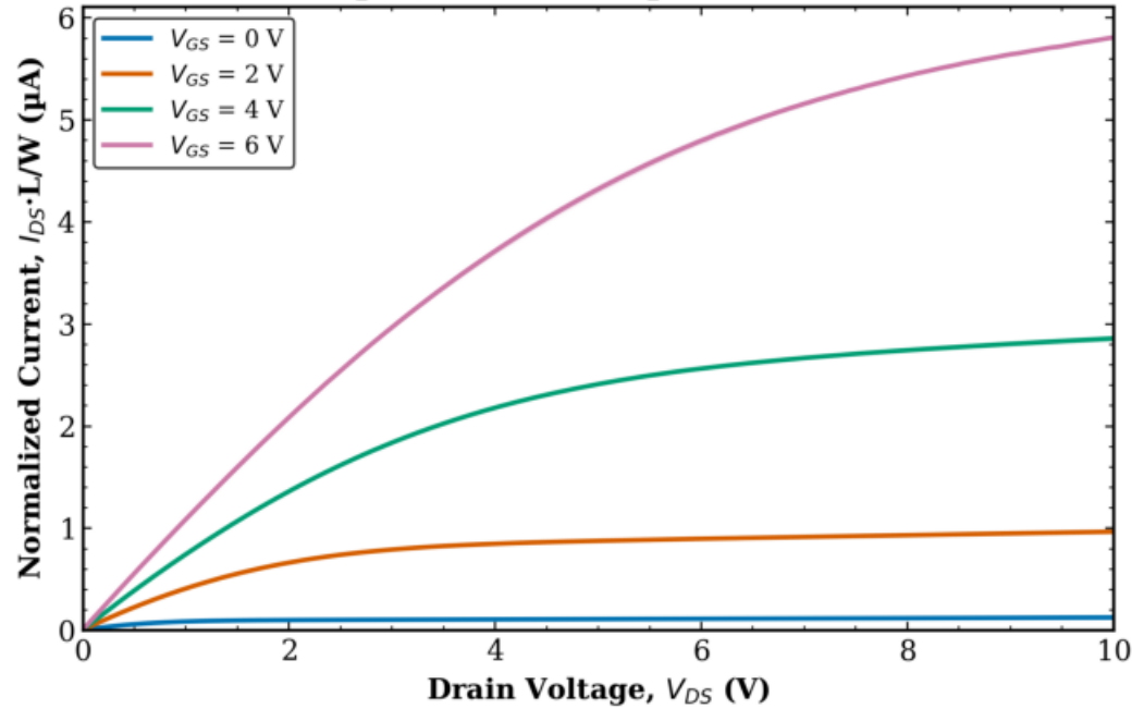
TFT1 Combined (Tr. 1 & 2) L = 10 \mu\text{m} , W = 1000 \mu\text{m} (normalized)
