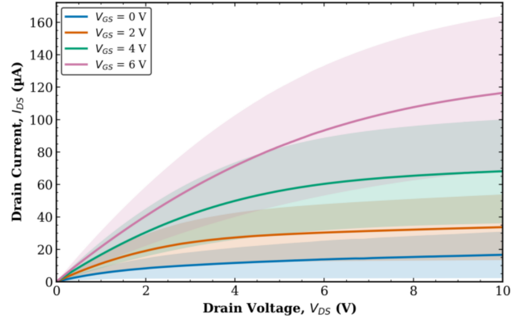
TFT1 Combined (Tr. 1 & 2) L = 10 \mu\text{m} , W = 100 \mu\text{m}
