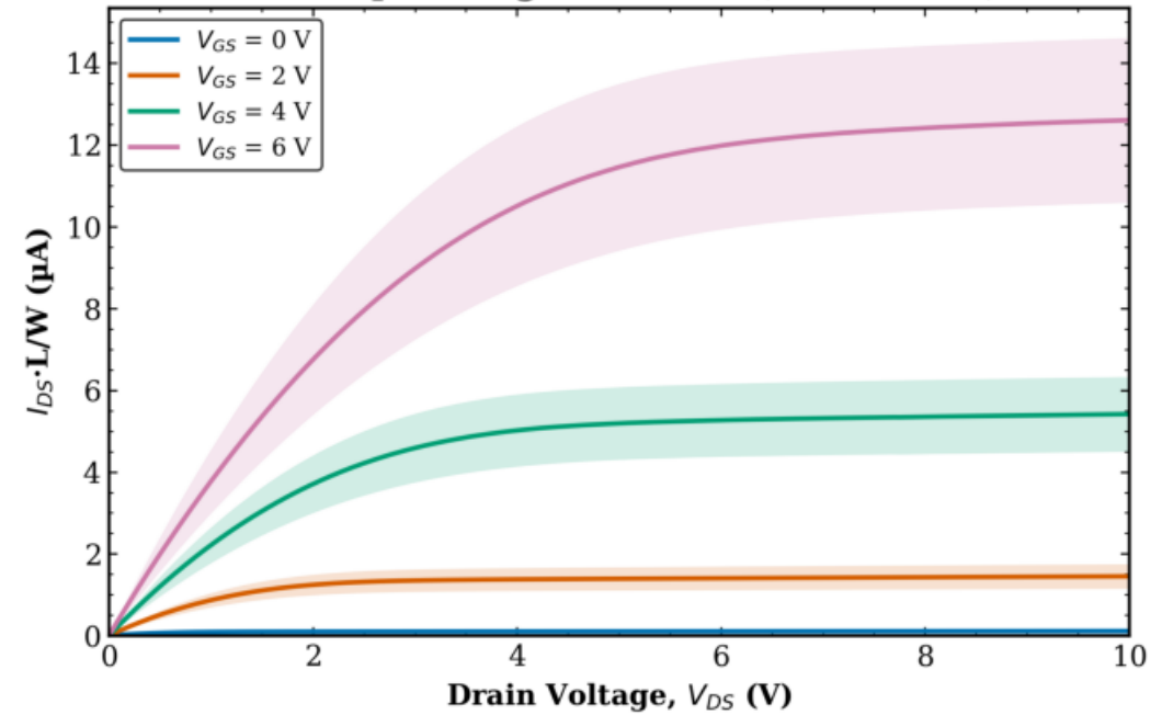
TFT1 Combined (Tr. 1 & 2) L = 40 \mu\text{m} - avg over all W (mean \pm std)
