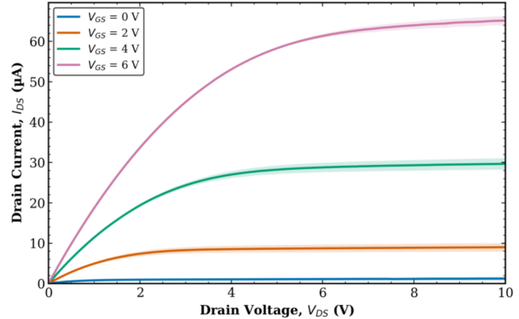
TFT1 Combined (Tr. 1 & 2) L = 20 \mu\text{m} , W = 100 \mu\text{m}
