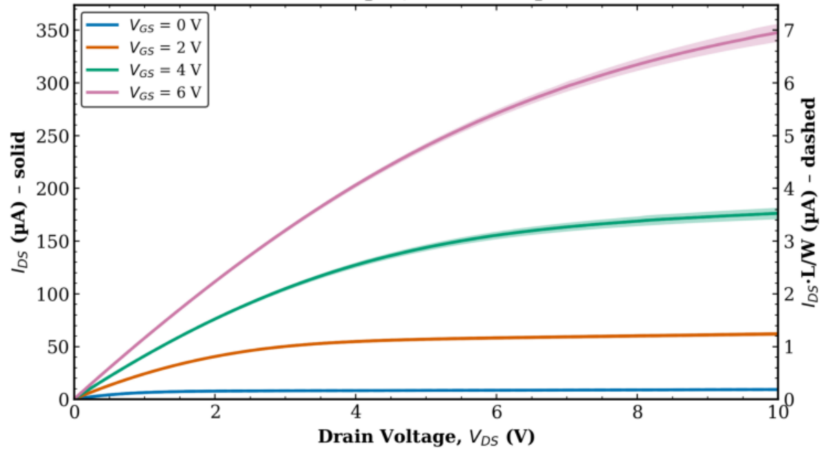
TFT1 Combined (Tr. 1 & 2) L = 10 \mu\text{m} , W = 500 \mu\text{m}
