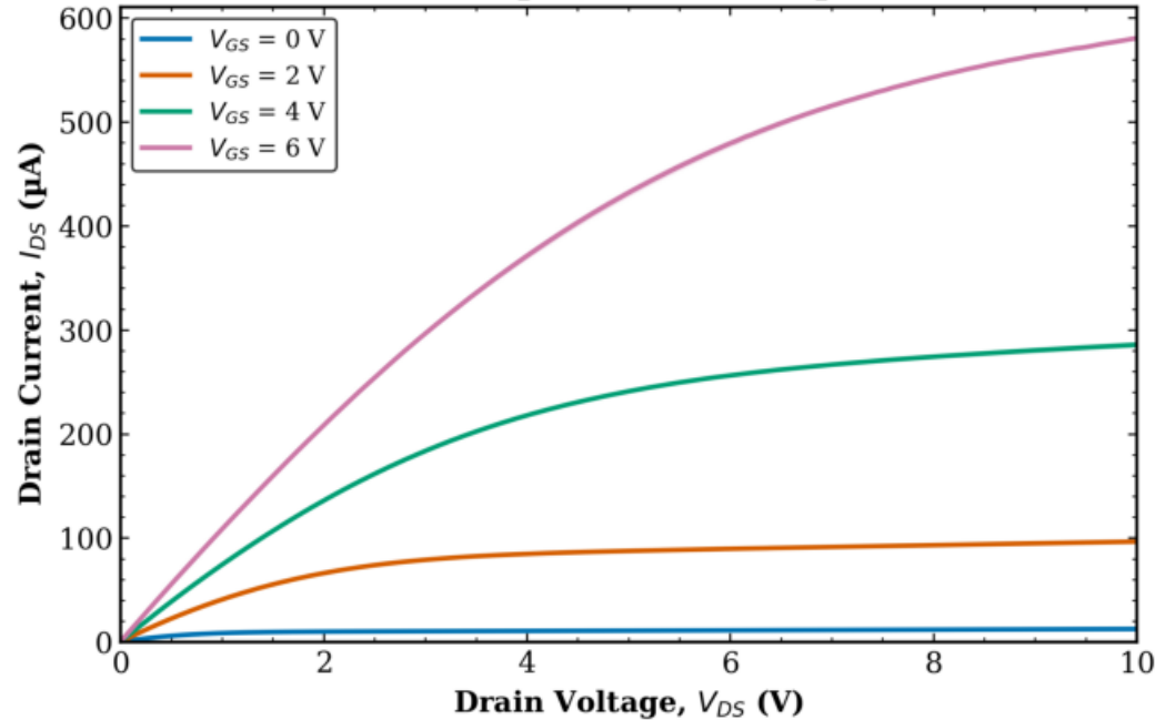
TFT1 Combined (Tr. 1 & 2) L = 10 \mu\text{m} , W = 1000 \mu\text{m}
