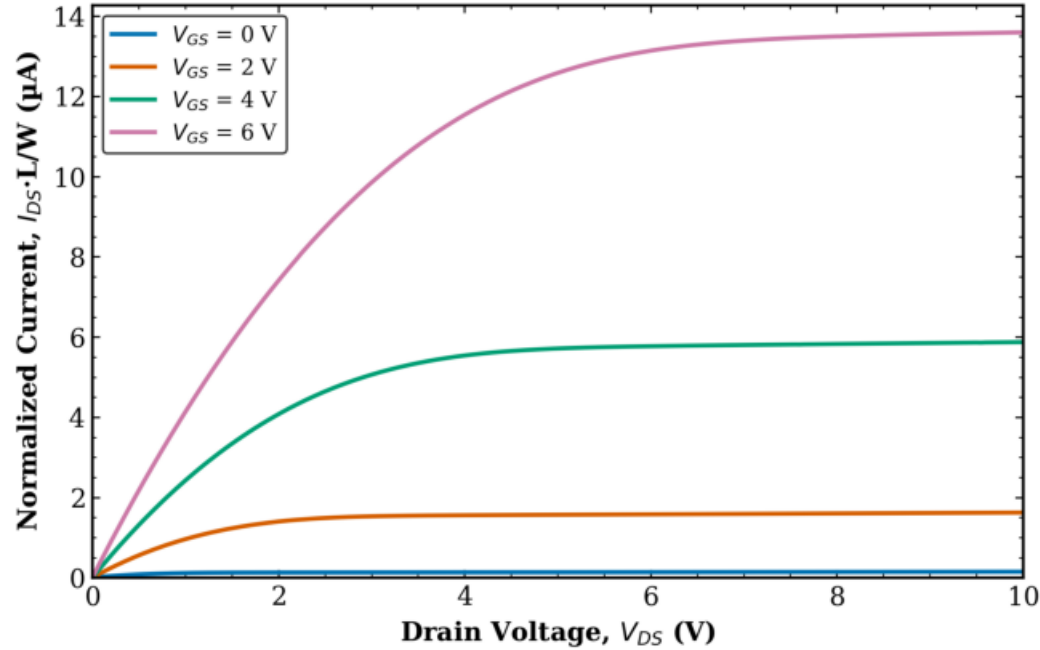
TFT1 Combined (Tr. 1 & 2) L = 80 \mu\text{m} , W = 500 \mu\text{m} (normalized)
