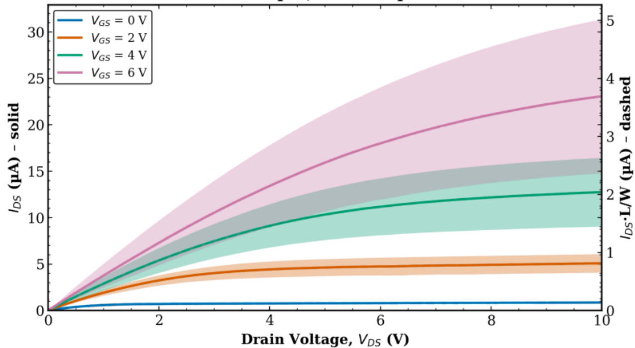
TFT1 Combined (Tr. 1 & 2) L = 8 \mu\text{m} , W = 50 \mu\text{m}
