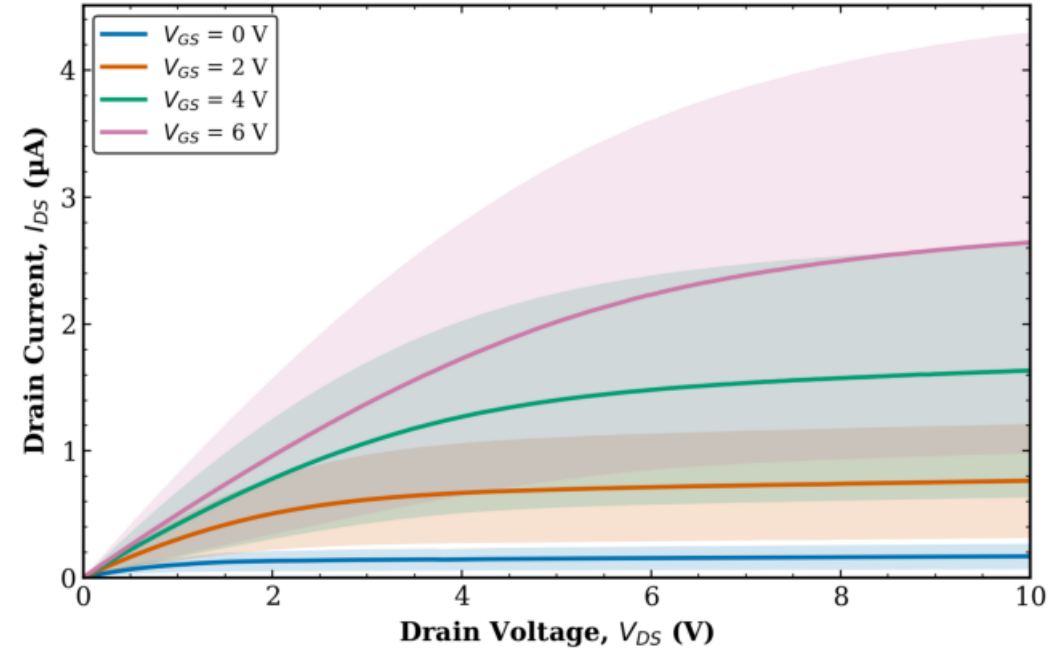
TFT1 Combined (Tr. 1 & 2) L = 8 \mu\text{m} , W = 10 \mu\text{m}
