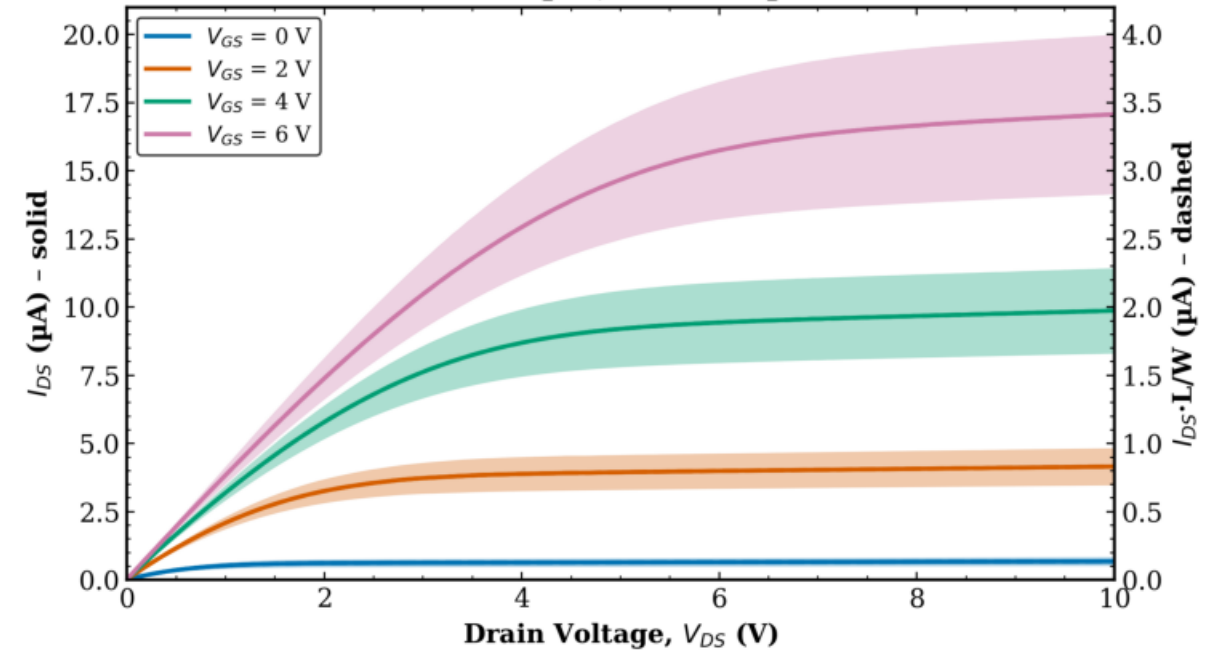
TFT1 Combined (Tr. 1 & 2) L = 10 \mu\text{m} , W = 50 \mu\text{m}
