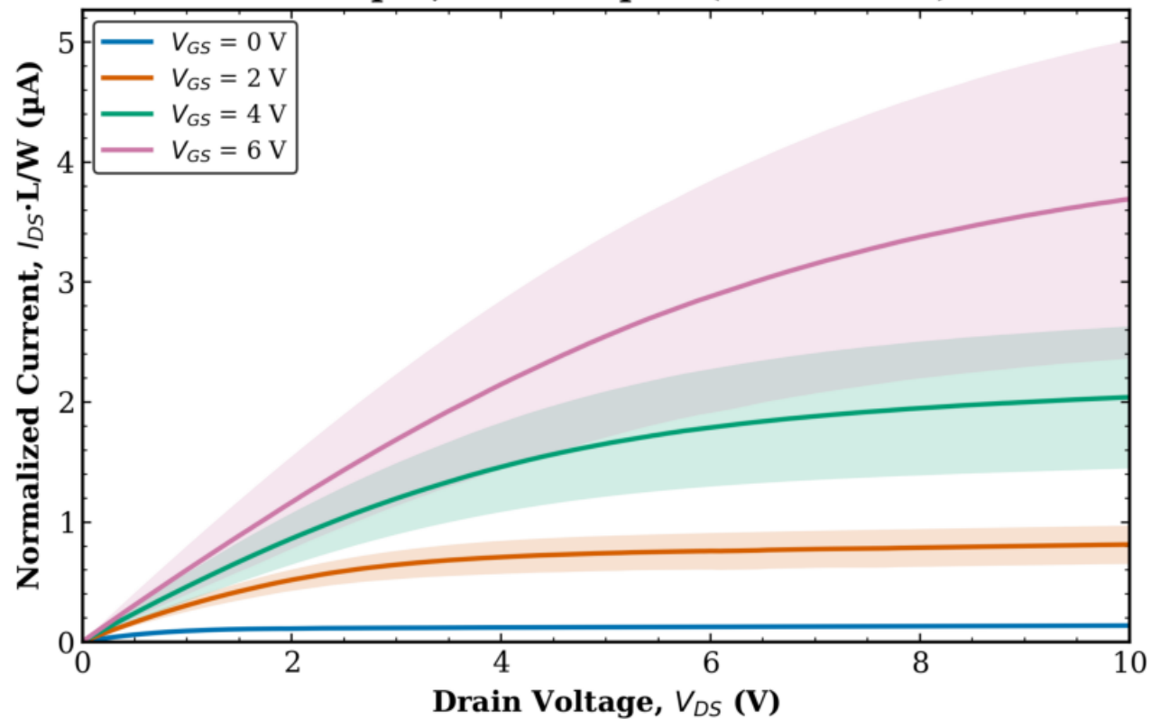
TFT1 Combined (Tr. 1 & 2) L = 8 \mu\text{m} , W = 50 \mu\text{m} (normalized)
