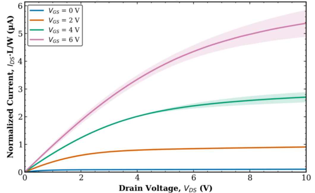
TFT1 Combined (Tr. 1 & 2) L = 8 \mu\text{m} , W = 1000 \mu\text{m} (normalized)
