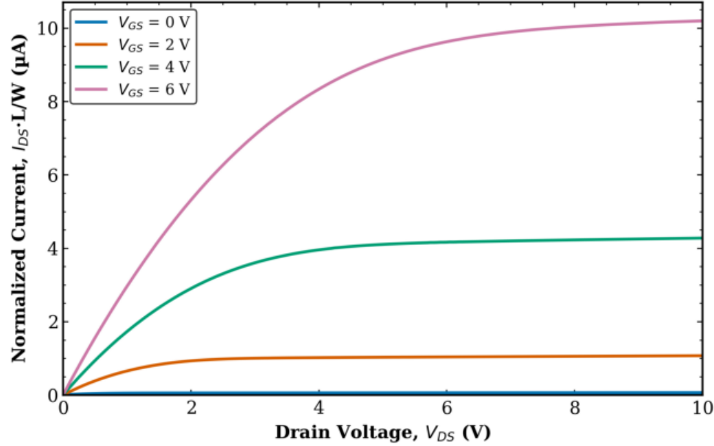
TFT1 Combined (Tr. 1 & 2) L = 40 \mu\text{m} , W = 500 \mu\text{m} (normalized)
