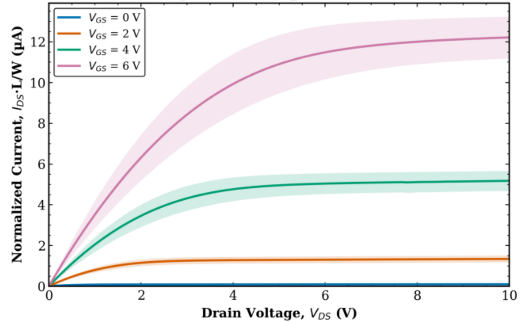
TFT1 Combined (Tr. 1 & 2) L = 40 \mu\text{m} , W = 50 \mu\text{m} (normalized)
