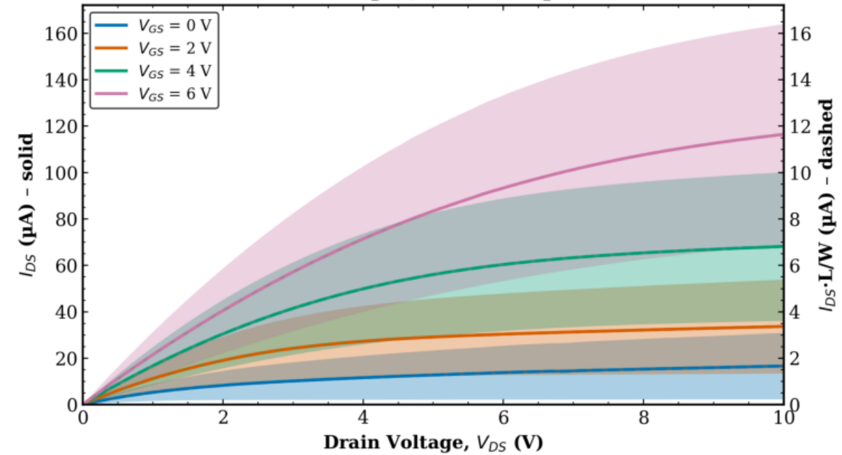
TFT1 Combined (Tr. 1 & 2) L = 10 \mu\text{m} , W = 100 \mu\text{m}
