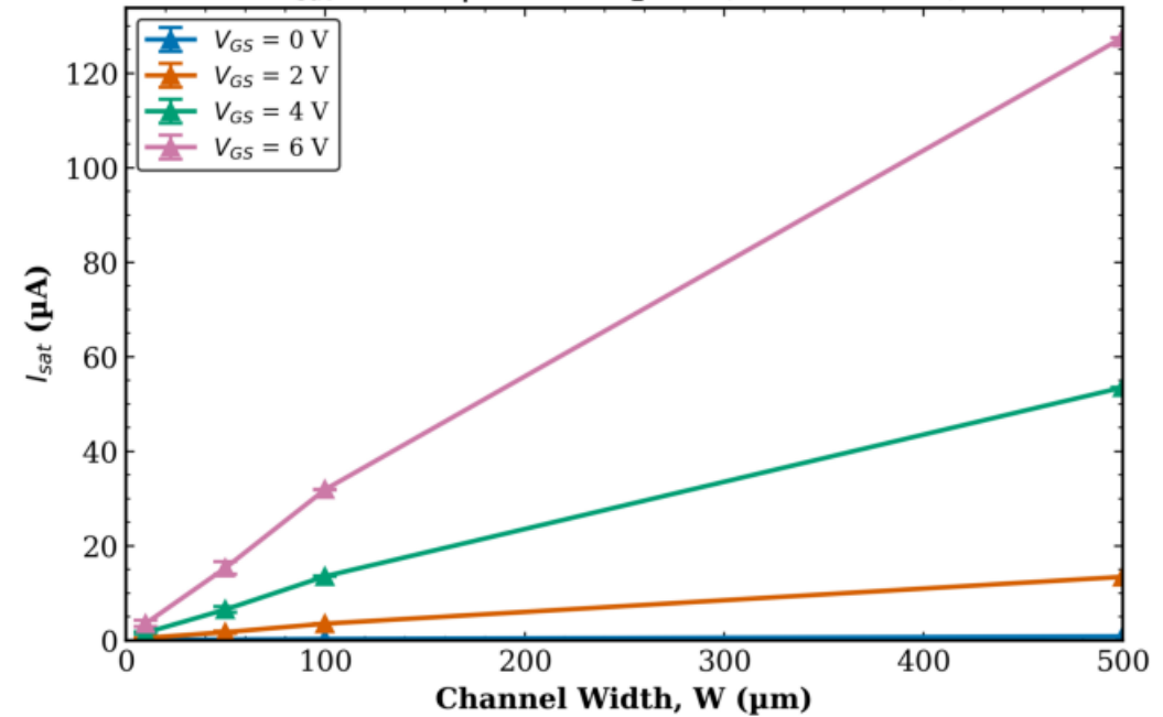
TFT1 Combined (Tr. 1 & 2) I_{sat} vs W | L = 40 \mu\text{m} (mean \pm std)
