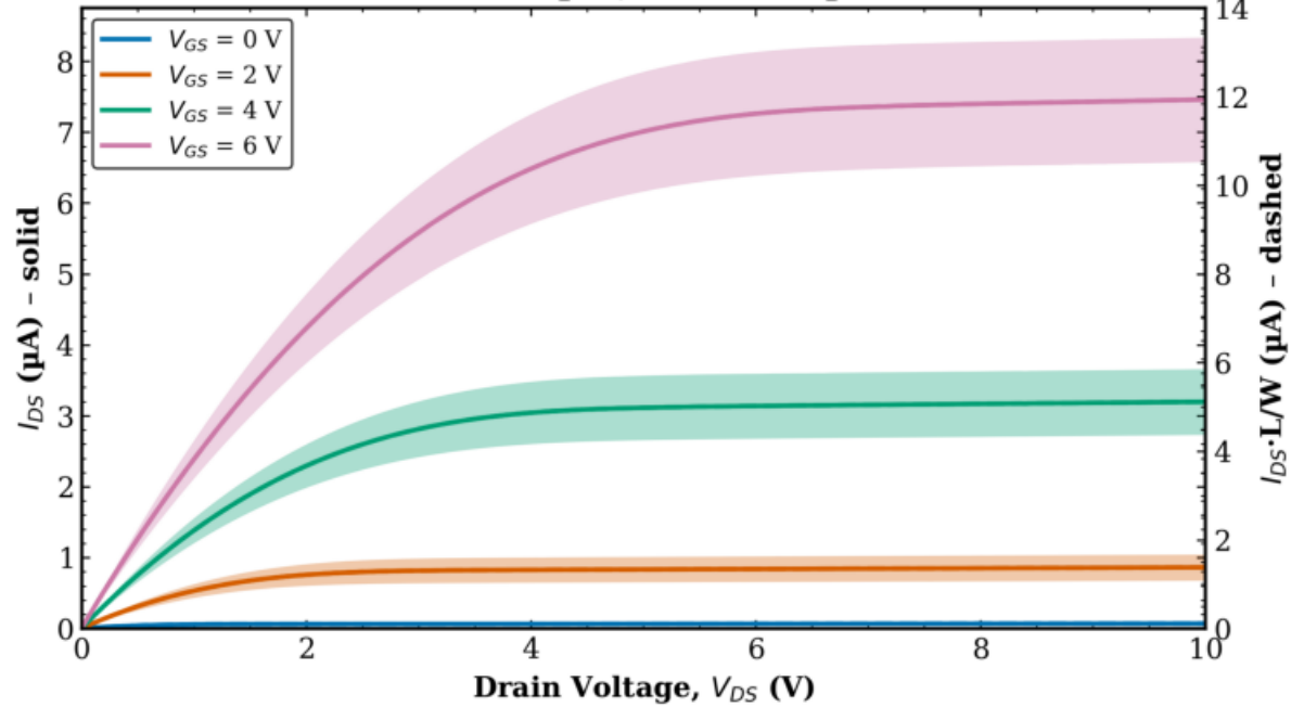
TFT1 Combined (Tr. 1 & 2) L = 160 \mu\text{m} , W = 100 \mu\text{m}
