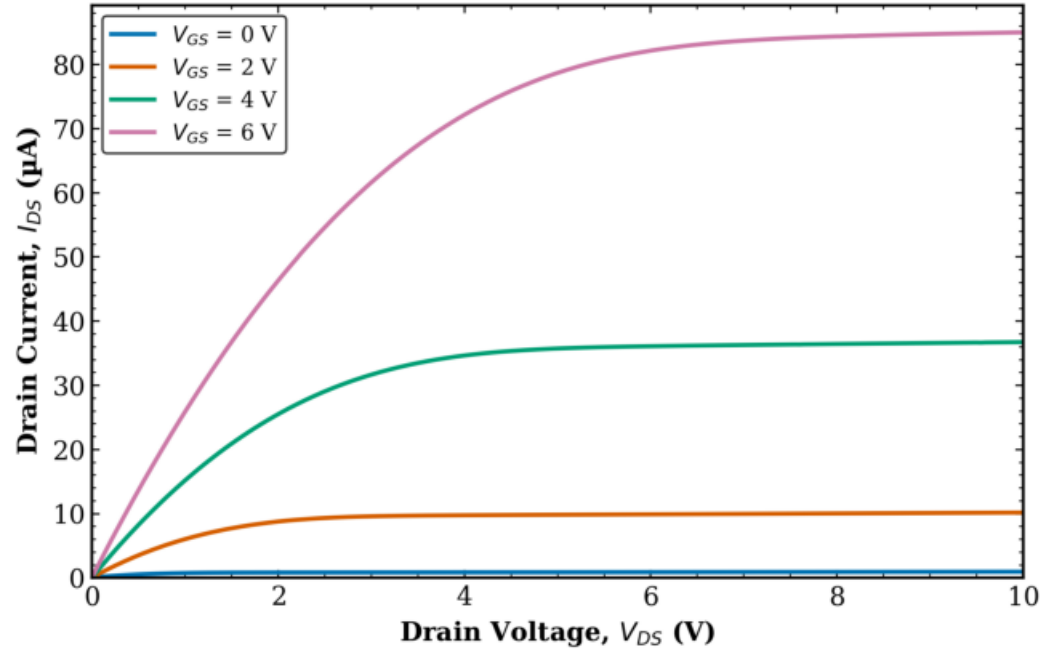
TFT1 Combined (Tr. 1 & 2) L = 80 \mu\text{m} , W = 500 \mu\text{m}
