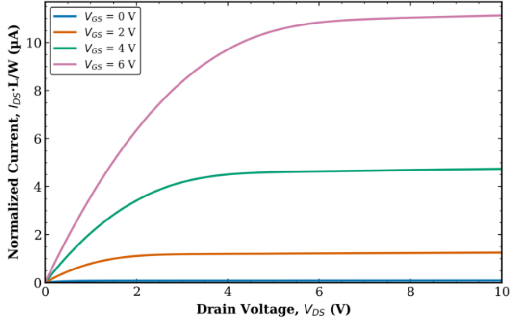
TFT1 Combined (Tr. 1 & 2) L = 80 \mu\text{m} , W = 100 \mu\text{m} (normalized)
