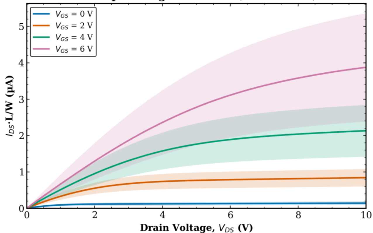
TFT1 Combined (Tr. 1 & 2) L = 8 \mu\text{m} - avg over all W (mean \pm std)
