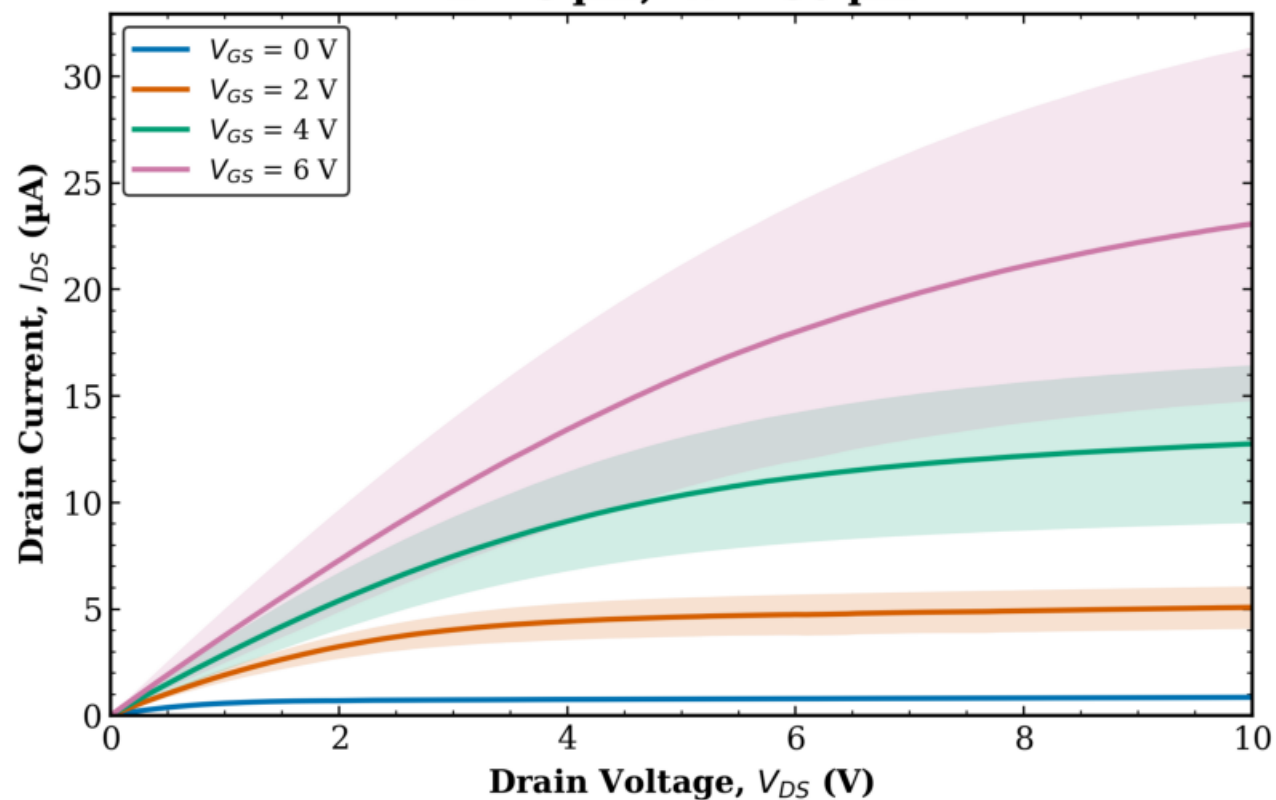
TFT1 Combined (Tr. 1 & 2) L = 8 \mu\text{m} , W = 50 \mu\text{m}
