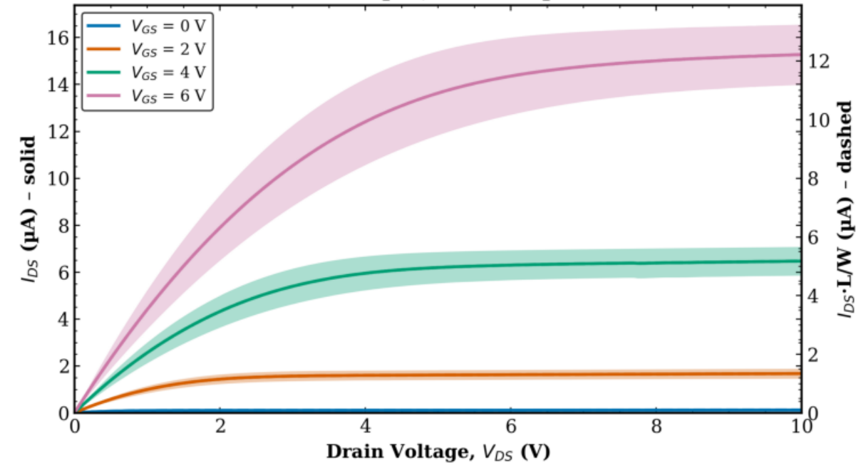
TFT1 Combined (Tr. 1 & 2) L = 40 \mu\text{m} , W = 50 \mu\text{m}
