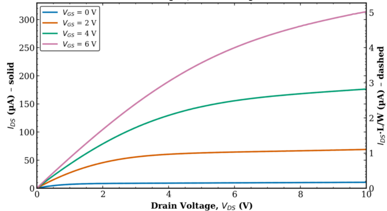
TFT1 Combined (Tr. 1 & 2) L = 8 \mu\text{m} , W = 500 \mu\text{m}
