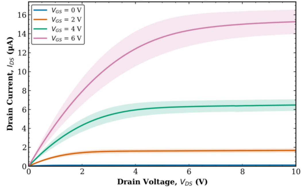
TFT1 Combined (Tr. 1 & 2) L = 40 \mu\text{m} , W = 50 \mu\text{m}
