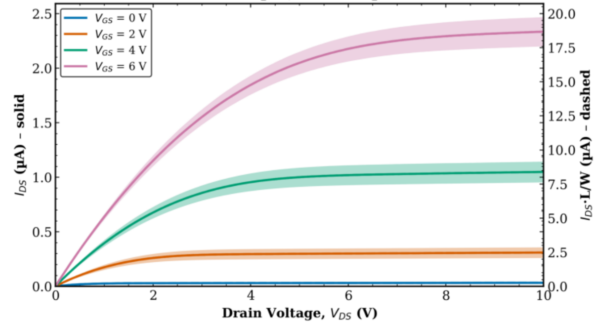
TFT1 Combined (Tr. 1 & 2) L = 80 \mu\text{m} , W = 10 \mu\text{m}
