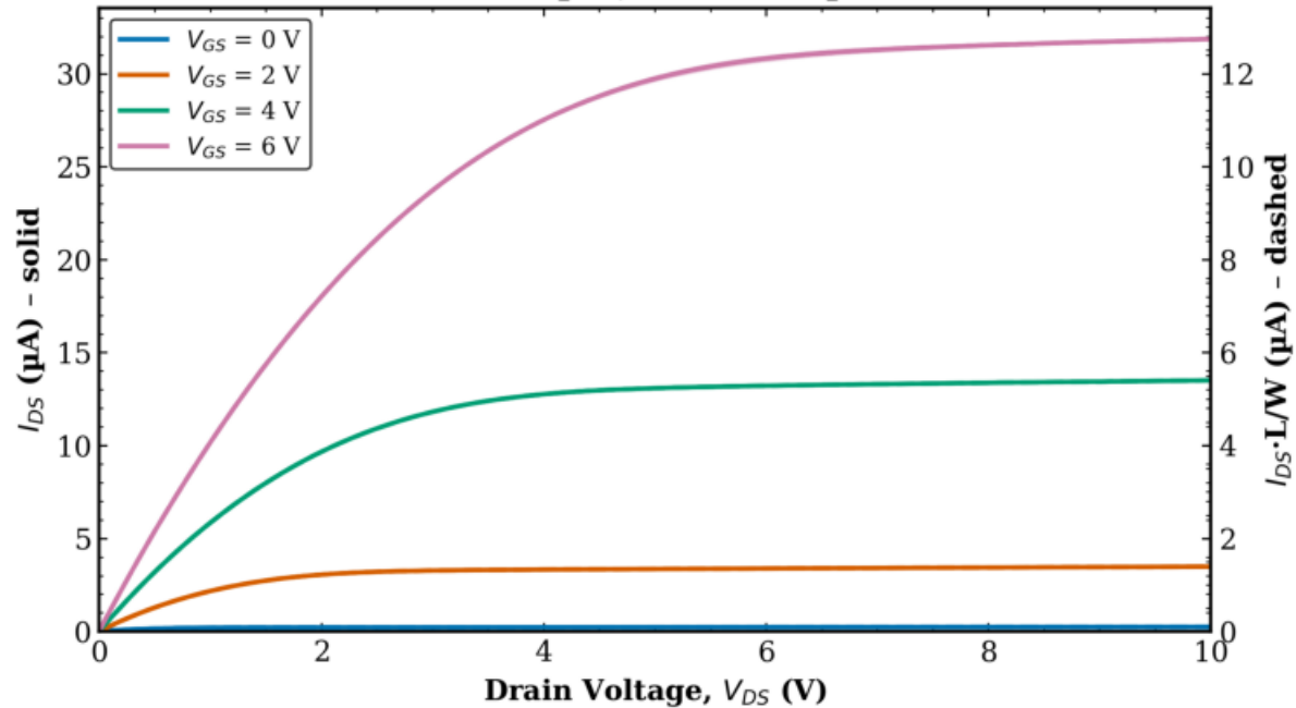
TFT1 Combined (Tr. 1 & 2) L = 40 \mu\text{m} , W = 100 \mu\text{m}
