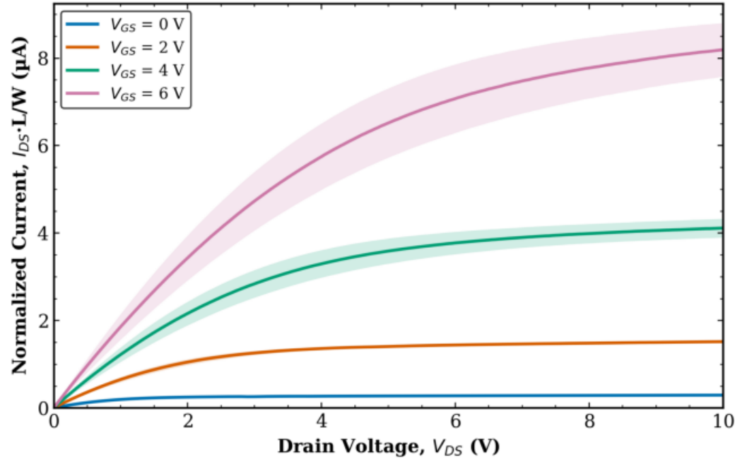
TFT1 Combined (Tr. 1 & 2) L = 10 \mu\text{m} , W = 10 \mu\text{m} (normalized)
