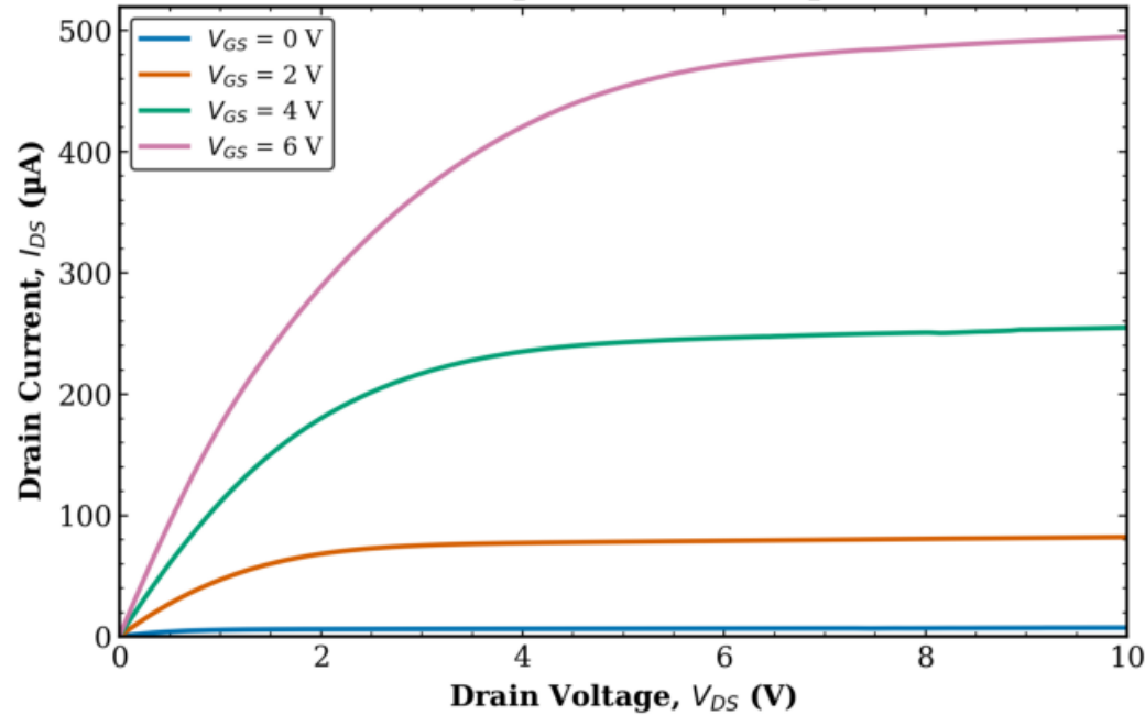
TFT1 Combined (Tr. 1 & 2) L = 20 \mu\text{m} , W = 1000 \mu\text{m}
