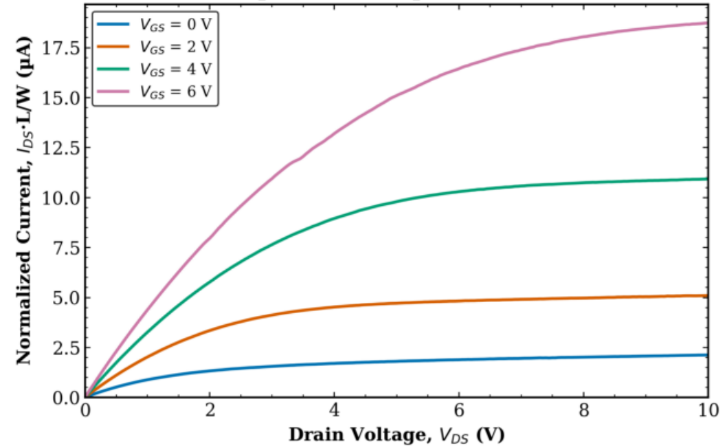
TFT1 Combined (Tr. 1 & 2) L = 20 \mu\text{m} , W = 50 \mu\text{m} (normalized)
