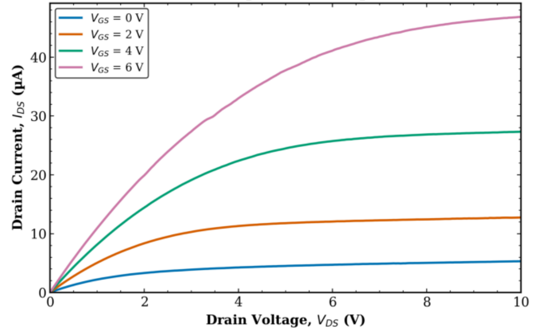
TFT1 Combined (Tr. 1 & 2) L = 20 \mu\text{m} , W = 50 \mu\text{m}
