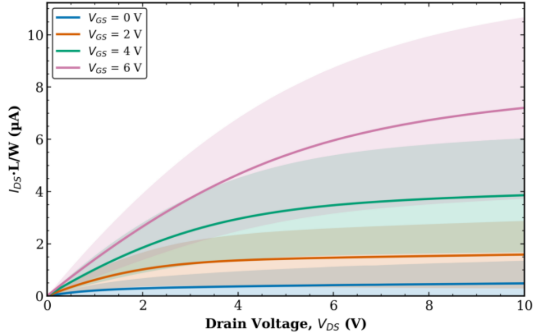
TFT1 Combined (Tr. 1 & 2) L = 10 \mu\text{m} - avg over all W (mean \pm std)
