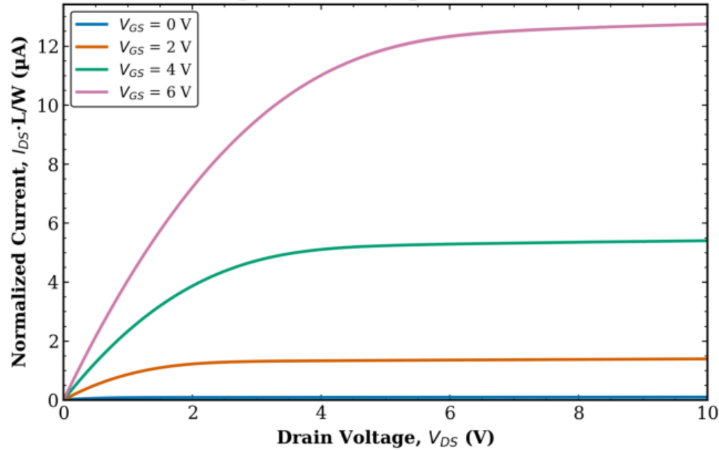
TFT1 Combined (Tr. 1 & 2) L = 40 \mu\text{m} , W = 100 \mu\text{m} (normalized)
