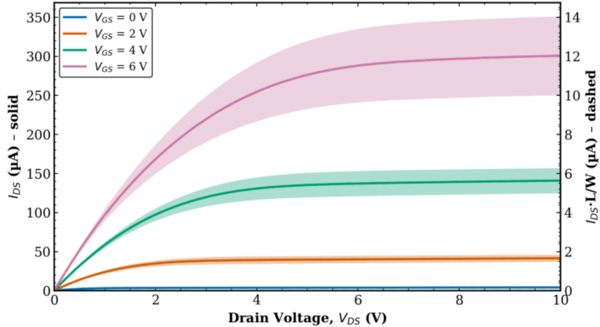
TFT1 Combined (Tr. 1 & 2) L = 20 \mu\text{m} , W = 500 \mu\text{m}
