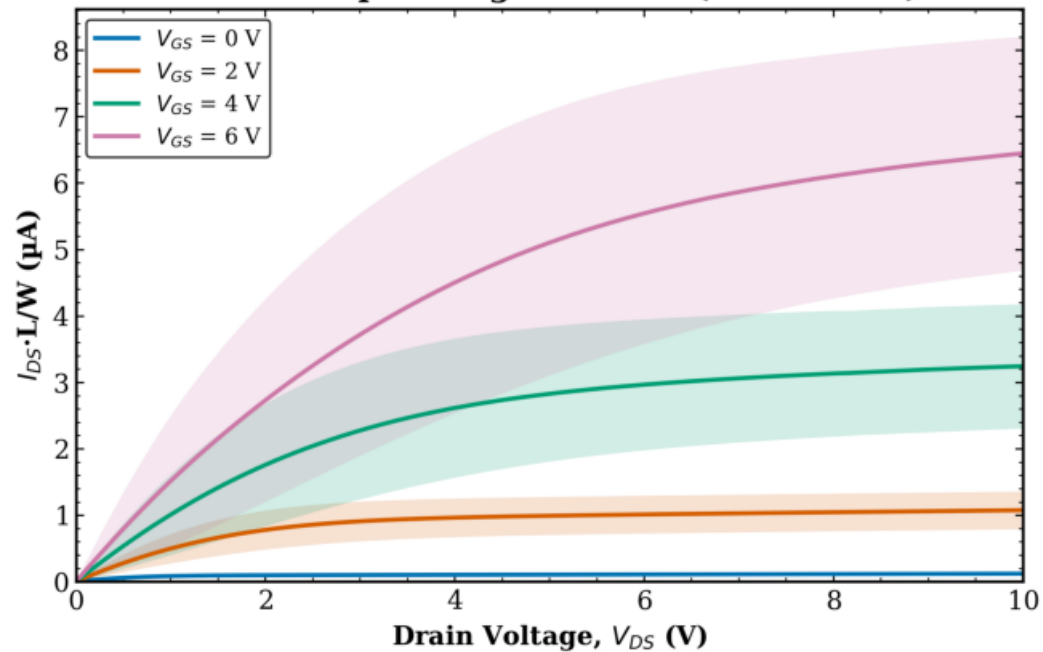
TFT1 Combined (Tr. 1 & 2) W = 1000 \mu\text{m} - avg over all L (mean \pm std)
