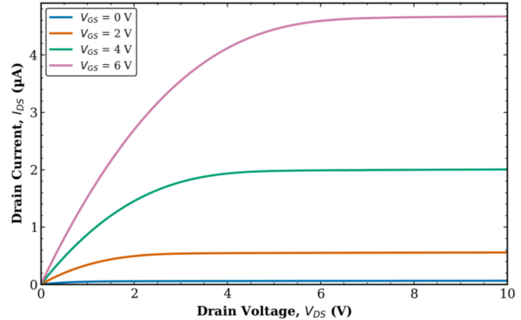
TFT1 Combined (Tr. 1 & 2) L = 160 \mu\text{m} , W = 50 \mu\text{m}
