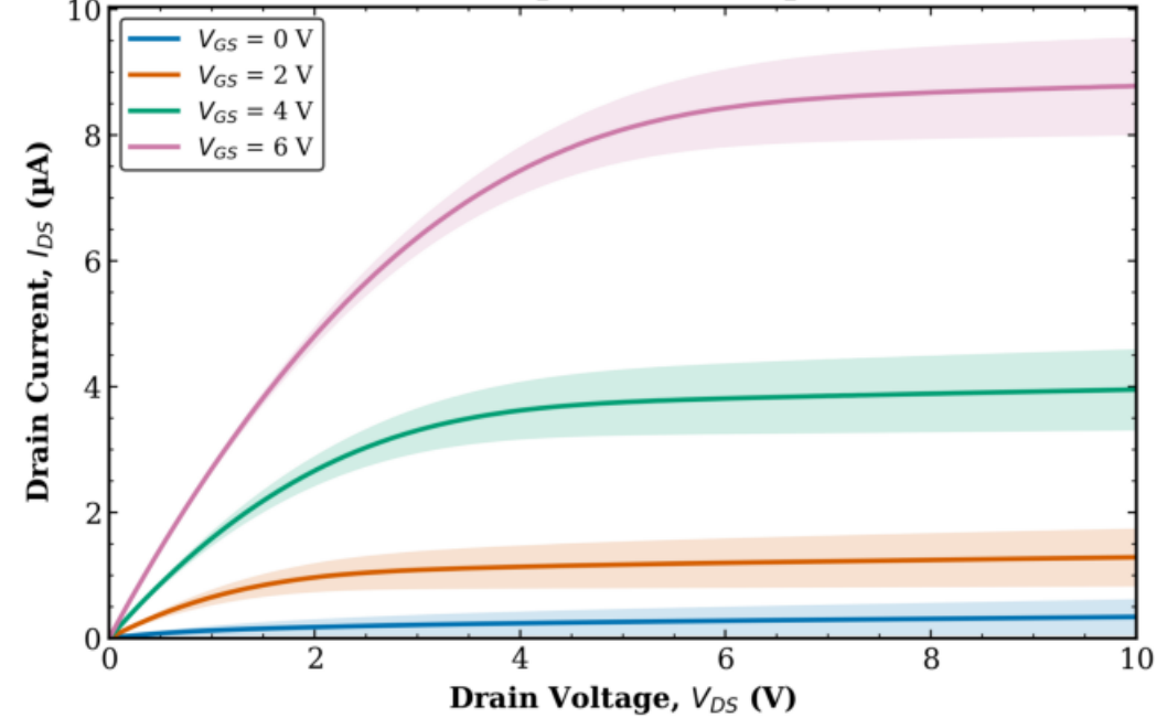
TFT1 Combined (Tr. 1 & 2) L = 80 \mu\text{m} , W = 50 \mu\text{m}
