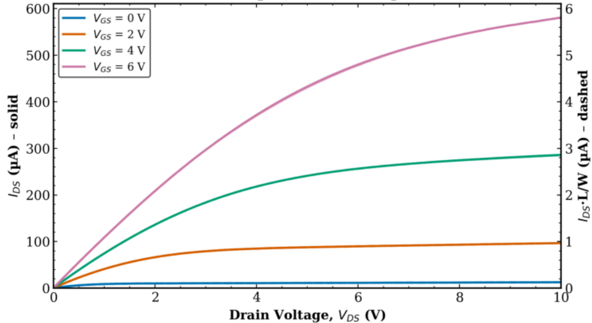
TFT1 Combined (Tr. 1 & 2) L = 10 \mu\text{m} , W = 1000 \mu\text{m}
