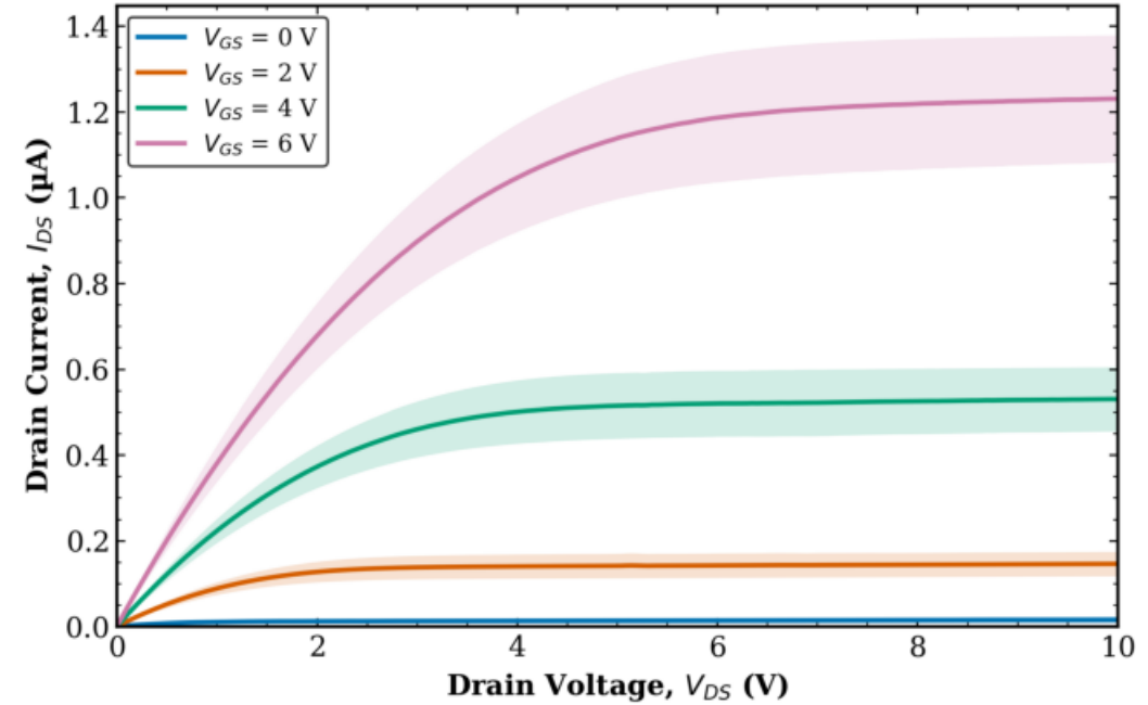
TFT1 Combined (Tr. 1 & 2) L = 160 \mu\text{m} , W = 10 \mu\text{m}
