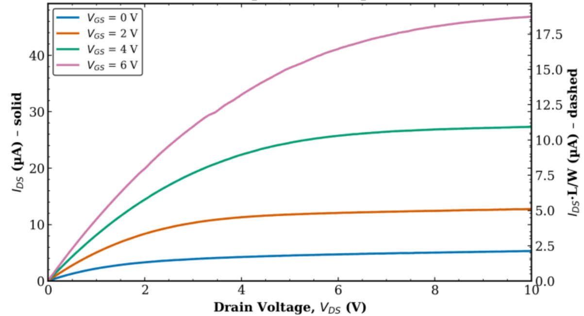
TFT1 Combined (Tr. 1 & 2) L = 20 \mu\text{m} , W = 50 \mu\text{m}
