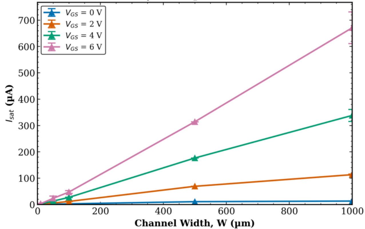
TFT1 Combined (Tr. 1 & 2) I_{sat} vs W | L = 8 \mu\text{m} (mean \pm std)
