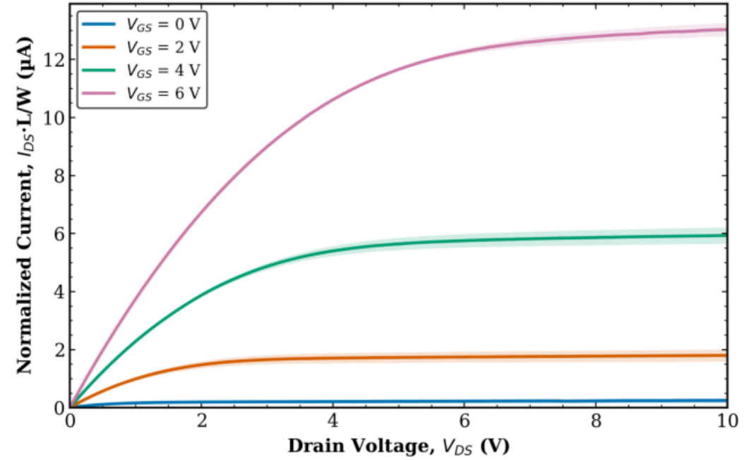
TFT1 Combined (Tr. 1 & 2) L = 20 \mu\text{m} , W = 100 \mu\text{m} (normalized)
