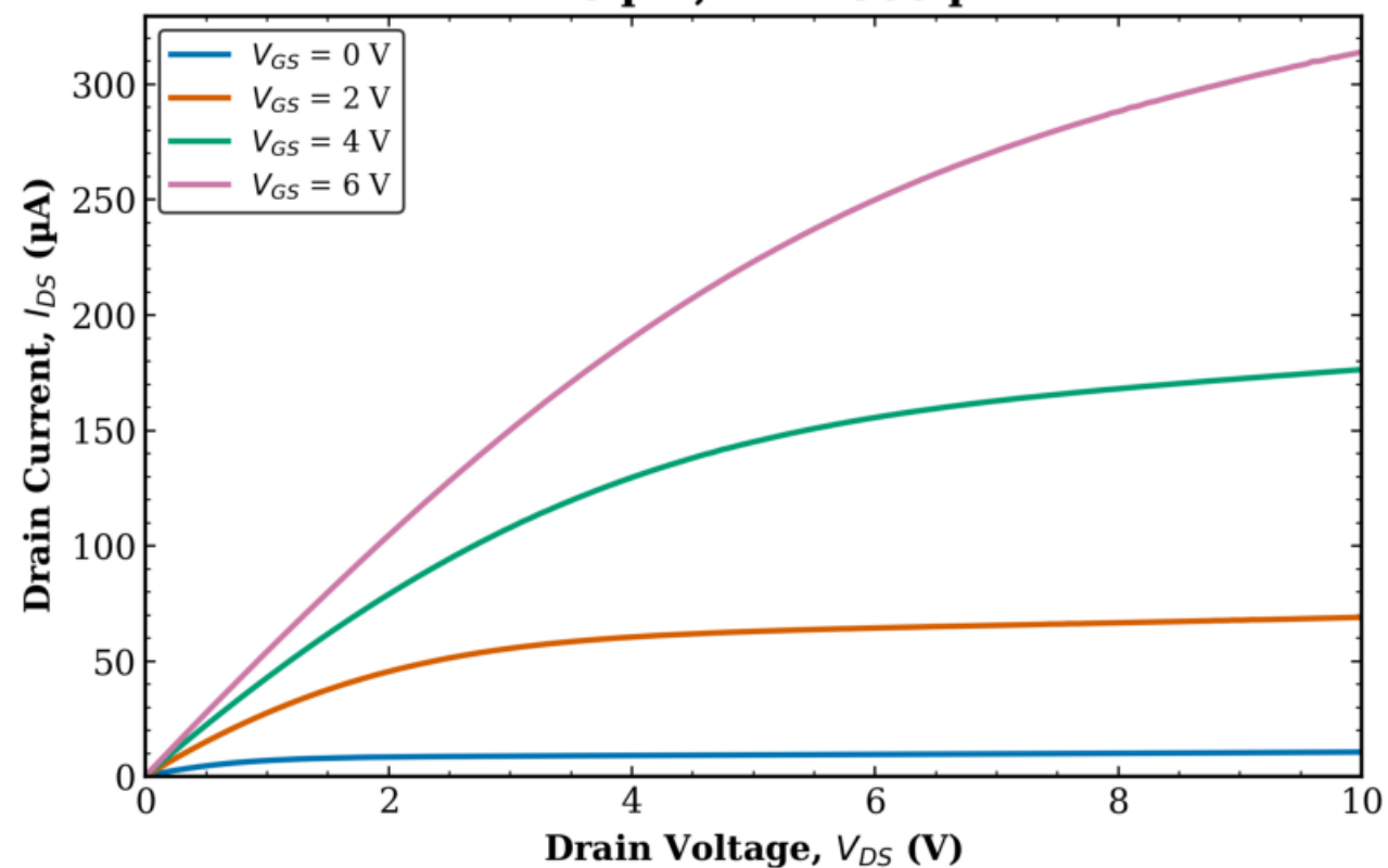
TFT1 Combined (Tr. 1 & 2) L = 8 \mu\text{m} , W = 500 \mu\text{m}
