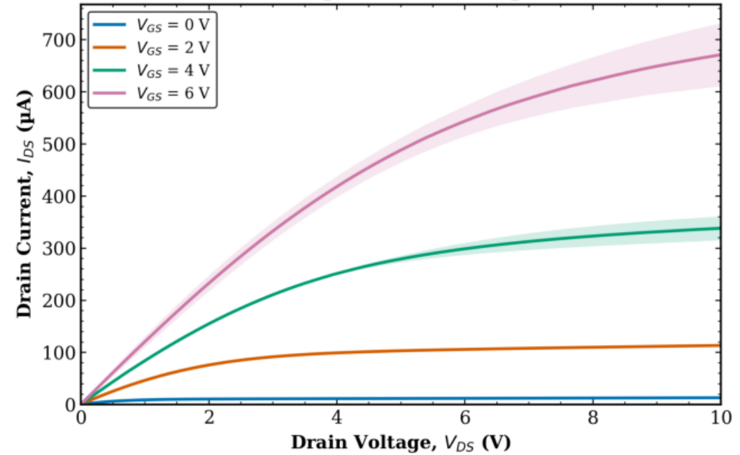
TFT1 Combined (Tr. 1 & 2) L = 8 \mu\text{m} , W = 1000 \mu\text{m}
