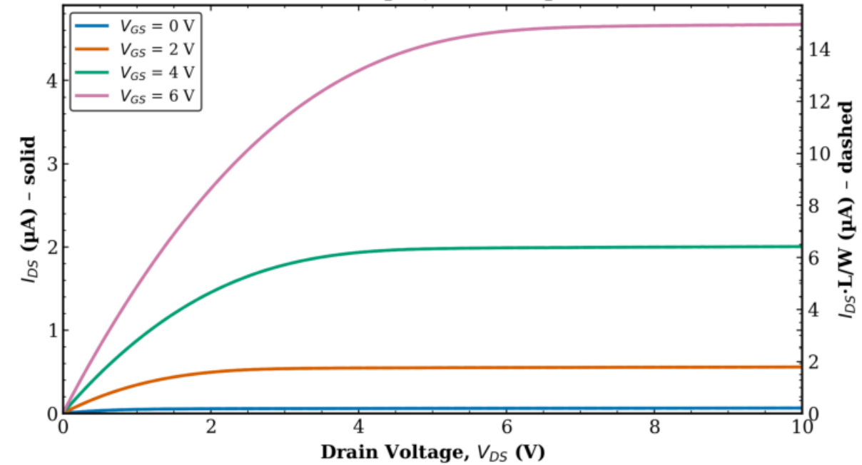
TFT1 Combined (Tr. 1 & 2) L = 160 \mu\text{m} , W = 50 \mu\text{m}
