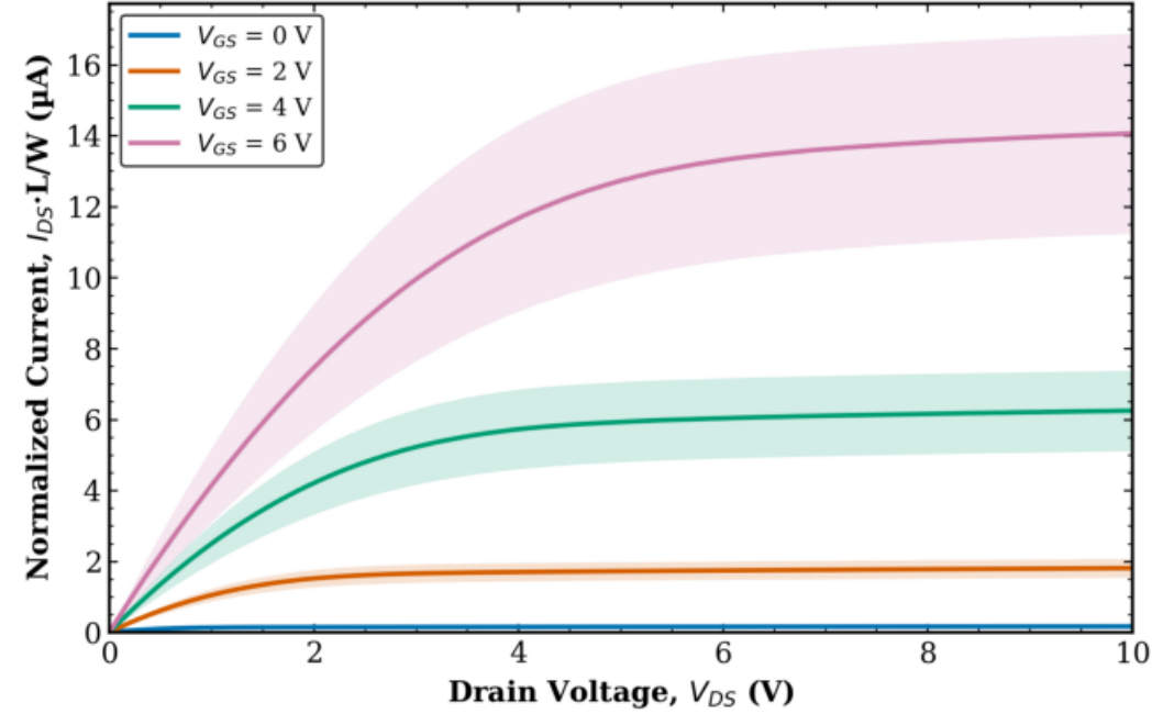
TFT1 Combined (Tr. 1 & 2) L = 40 \mu\text{m} , W = 10 \mu\text{m} (normalized)
