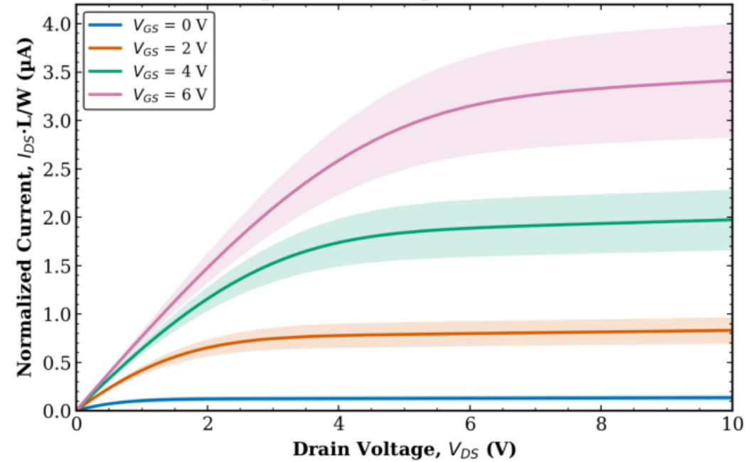
TFT1 Combined (Tr. 1 & 2) L = 10 \mu\text{m} , W = 50 \mu\text{m} (normalized)
