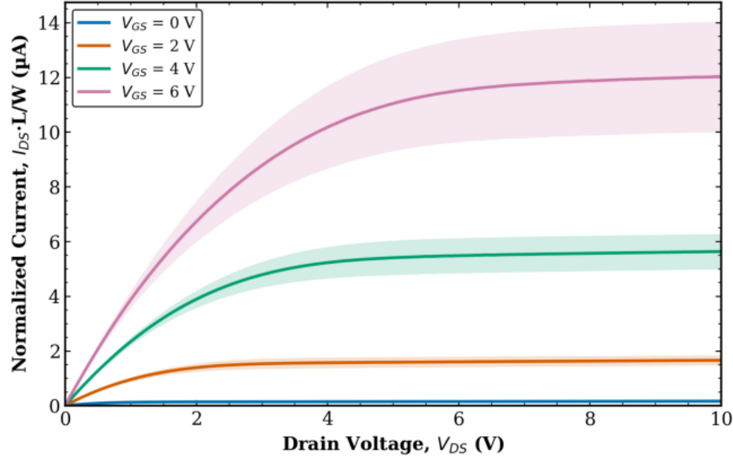
TFT1 Combined (Tr. 1 & 2) L = 20 \mu\text{m} , W = 500 \mu\text{m} (normalized)
