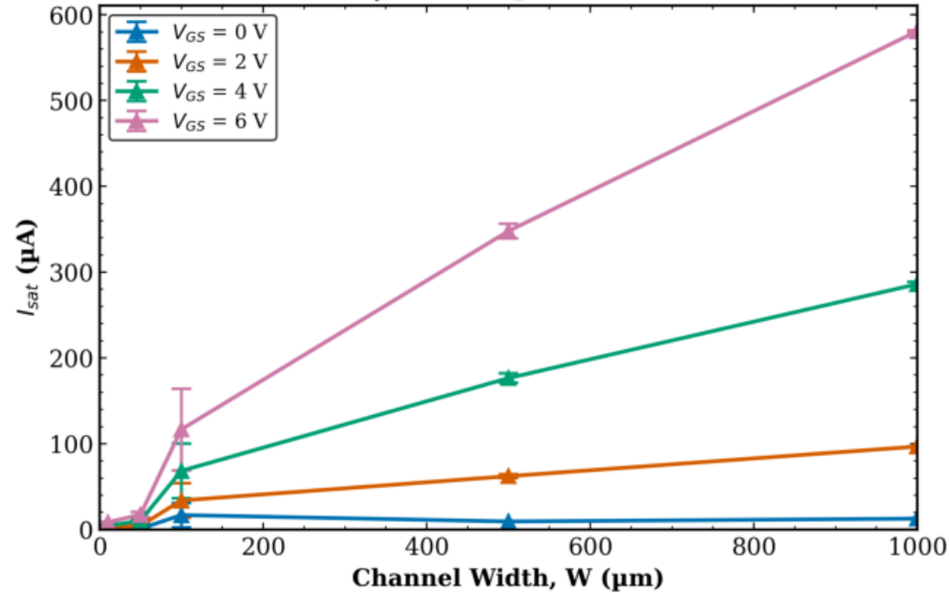
TFT1 Combined (Tr. 1 & 2) I_{sat} vs W | L = 10 \mu\text{m} (mean \pm std)
