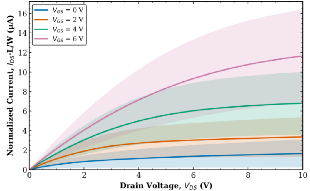
TFT1 Combined (Tr. 1 & 2) L = 10 \mu\text{m} , W = 100 \mu\text{m} (normalized)
