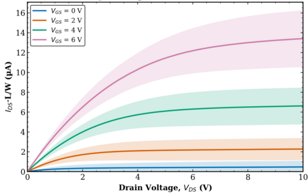
TFT1 Combined (Tr. 1 & 2) L = 20 \mu\text{m} - avg over all W (mean \pm std)
