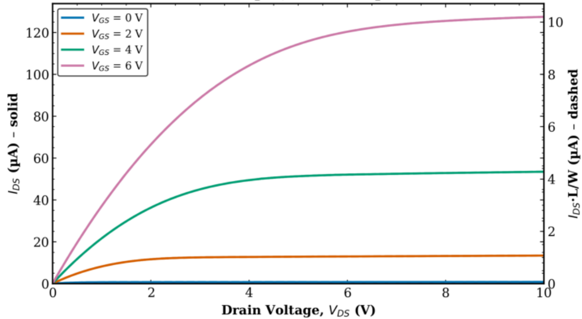
TFT1 Combined (Tr. 1 & 2) L = 40 \mu\text{m} , W = 500 \mu\text{m}
