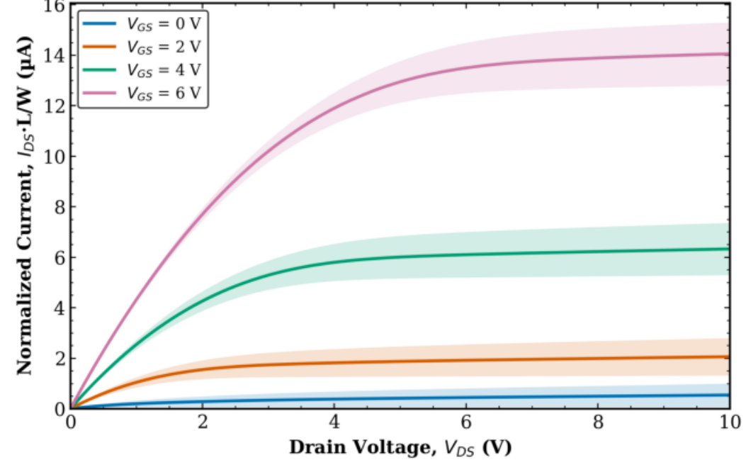
TFT1 Combined (Tr. 1 & 2) L = 80 \mu\text{m} , W = 50 \mu\text{m} (normalized)
