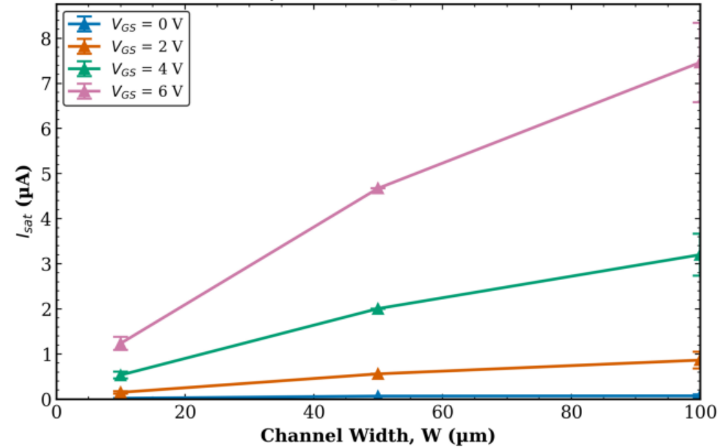
TFT1 Combined (Tr. 1 & 2) I_{sat} vs W | L = 160 \mu\text{m} (mean \pm std)
