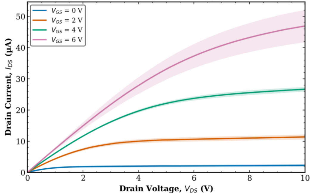
TFT1 Combined (Tr. 1 & 2) L = 8 \mu\text{m} , W = 100 \mu\text{m}
