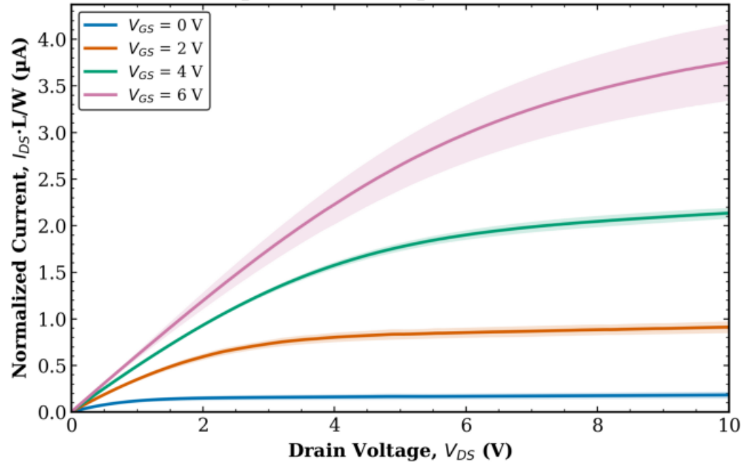
TFT1 Combined (Tr. 1 & 2) L = 8 \mu\text{m} , W = 100 \mu\text{m} (normalized)
